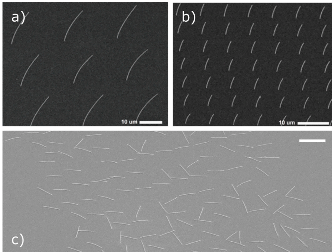
Fig. 3. SEM images of the written nanopillar samples on a 45° sample holder, showing a) maximum aspect ratio of approximately 100, having a pillar diameter of 254 \text{ nm} \pm 17 \text{ nm} and a height of 25 \text{ } \mu\text{m} ; b) shows the pillar array that was written to mimic the primary cilium in the collecting duct. With a diameter of 251 \text{ nm} \pm 22 \text{ nm} , a height of 7.5 \text{ } \mu\text{m} \pm 116 \text{ nm} , and spacing of 8 \text{ } \mu\text{m} the written cilia do indeed mimic the renal cilia. c) Without critical point drying, the large nanopillars collapse to the substrate during drying due to surface tension forces. All scale bars are 10 \text{ } \mu\text{m} .
