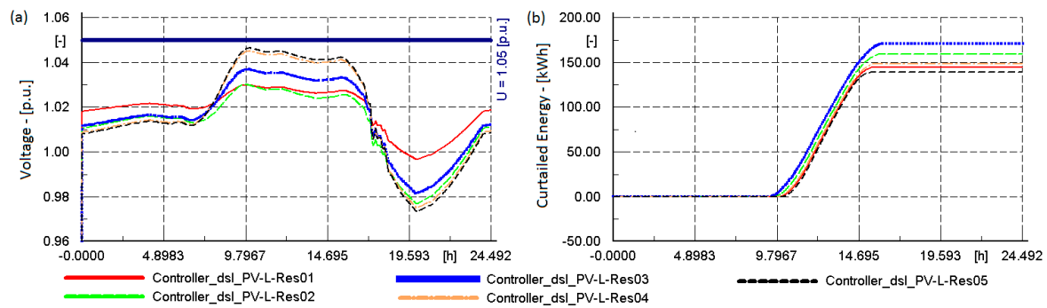
Figure 11. (a) Voltage profiles at PCC of each inverter with CC1; and (b) curtailed energy from each inverter.
