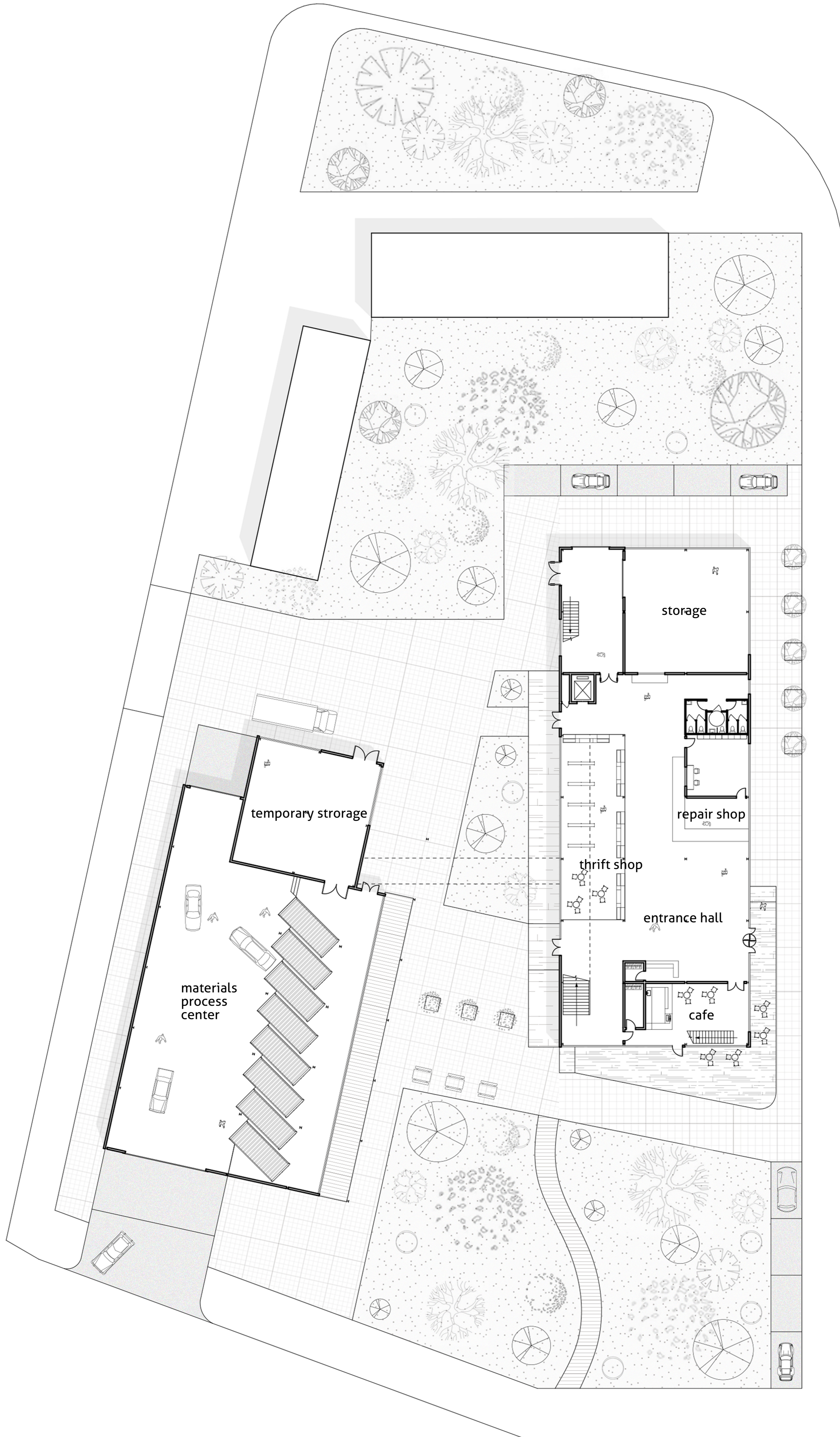
Ground floor 1:200
