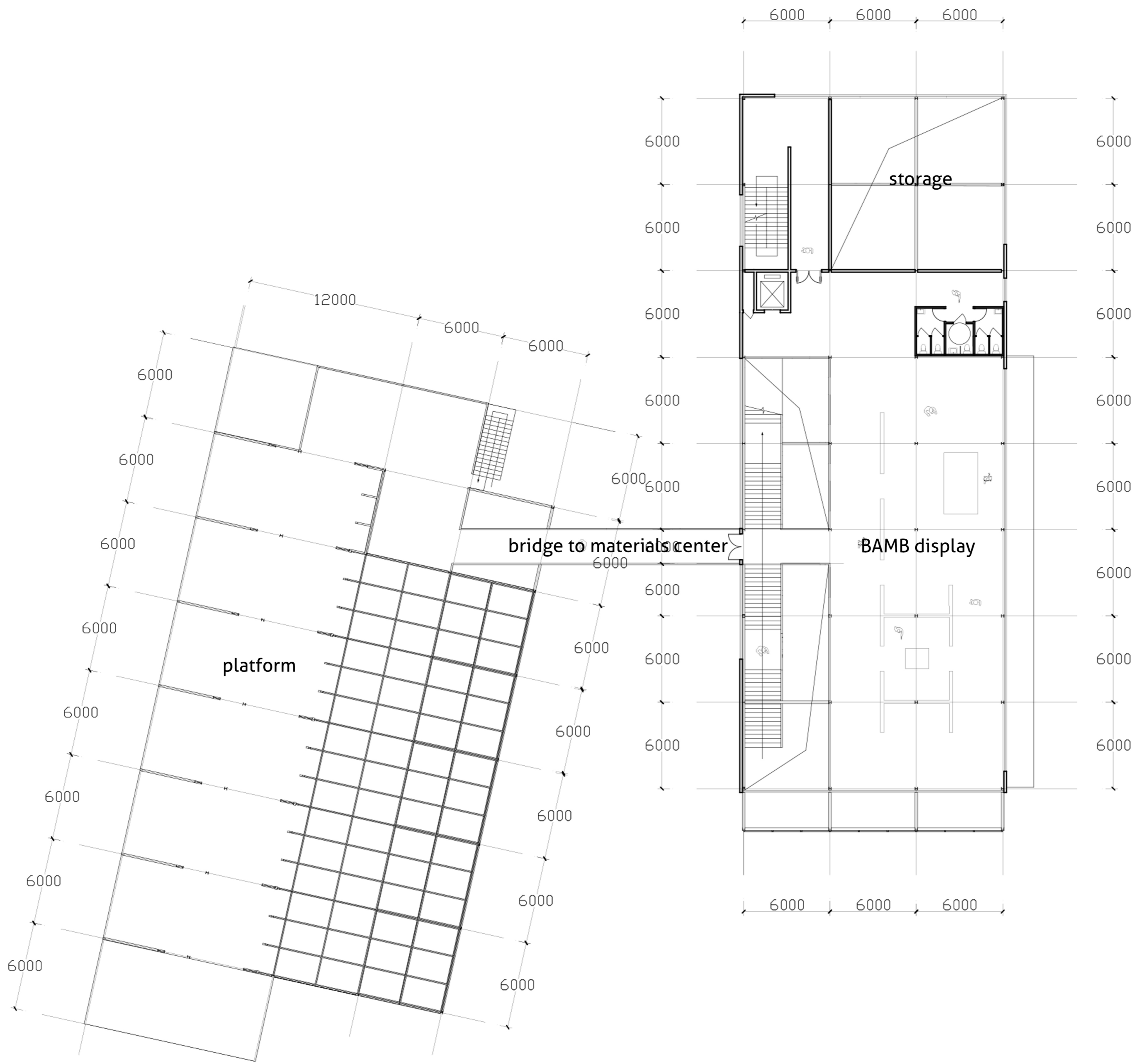
First floor 1:200
