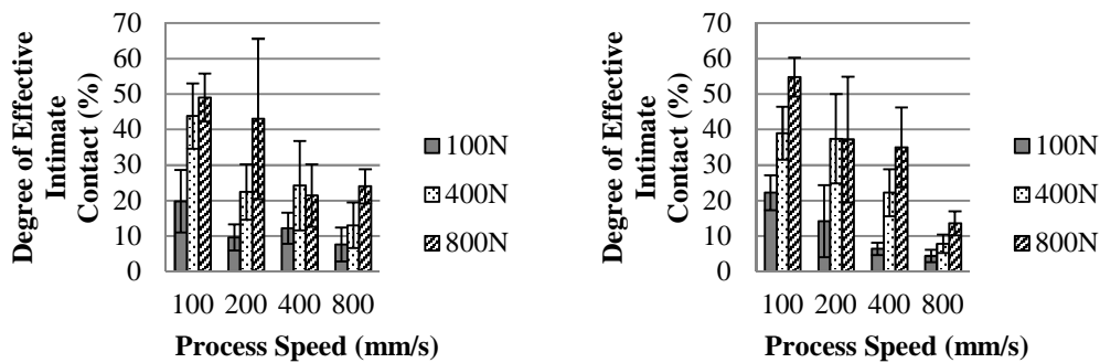
Figure 5. Degree of effective intimate contact vs. placement speed and compaction force- Tool temperature: 155 °C. Left: aimed nip point temperature 380 °C, right: aimed nip point temperature 400 °C. Error bars indicate standard deviation.
