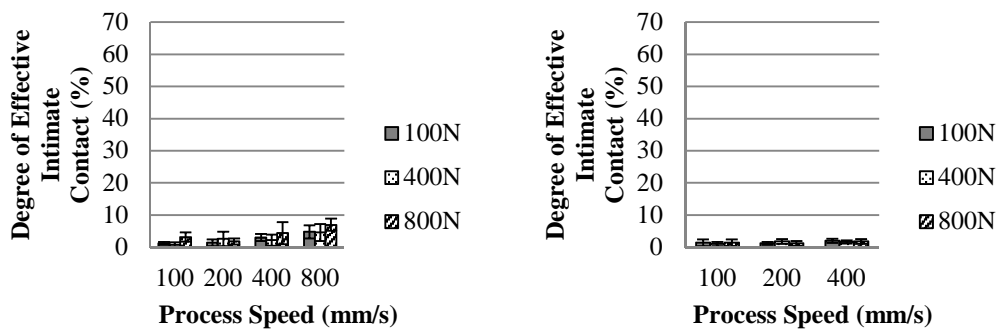
Figure 4. Degree of effective intimate contact vs. placement speed and compaction force- Tool temperature: 20 °C. Left: aimed nip point temperature 380 °C, right: aimed nip point temperature 400 °C. Error bars indicate standard deviation.
