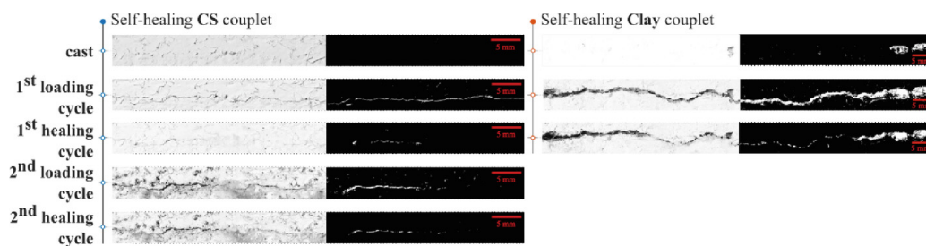
Fig. 4. Fully cracked self-healing couplets before and after multiple cracking-healing cycles.
