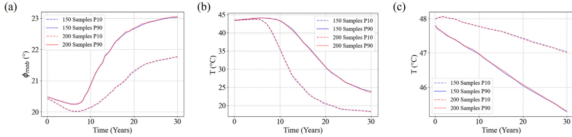
Fig. 15. The uncertainty boundary curves (P10 and P90) of 150 and 200 samples from the optimization: (a) stability of the drift, (b) temperature at the drift, (c) temperature at the production well.
