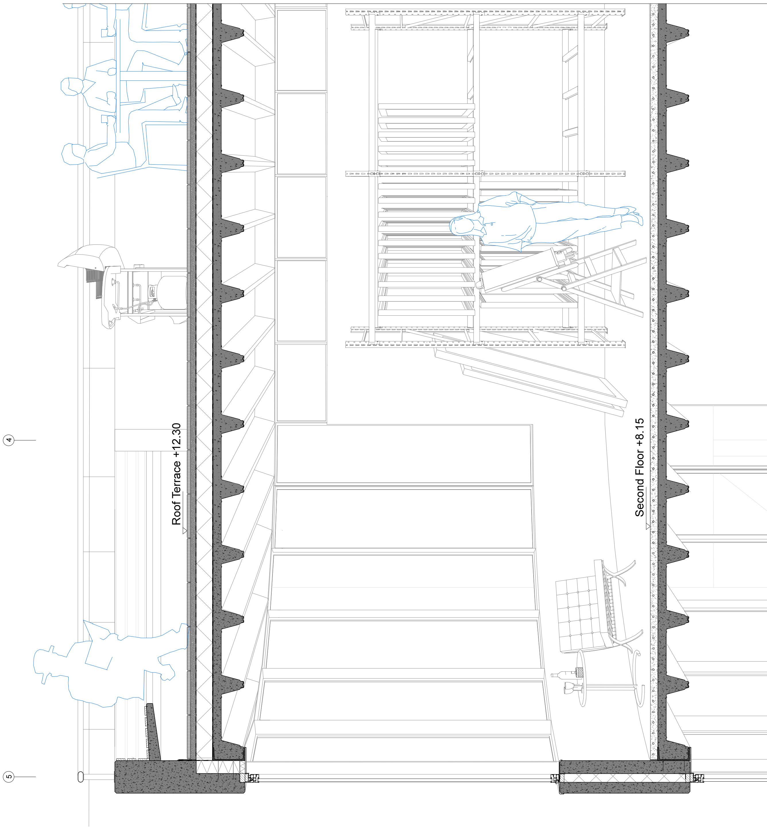
Section L1
