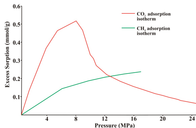
Figure 4. CO 2 vs CH 4 excess sorption, as a function of pressure for a high-TOC shale from Irati Formation, Brazil (redrawn and adapted from Weniger et al. 130 ).
