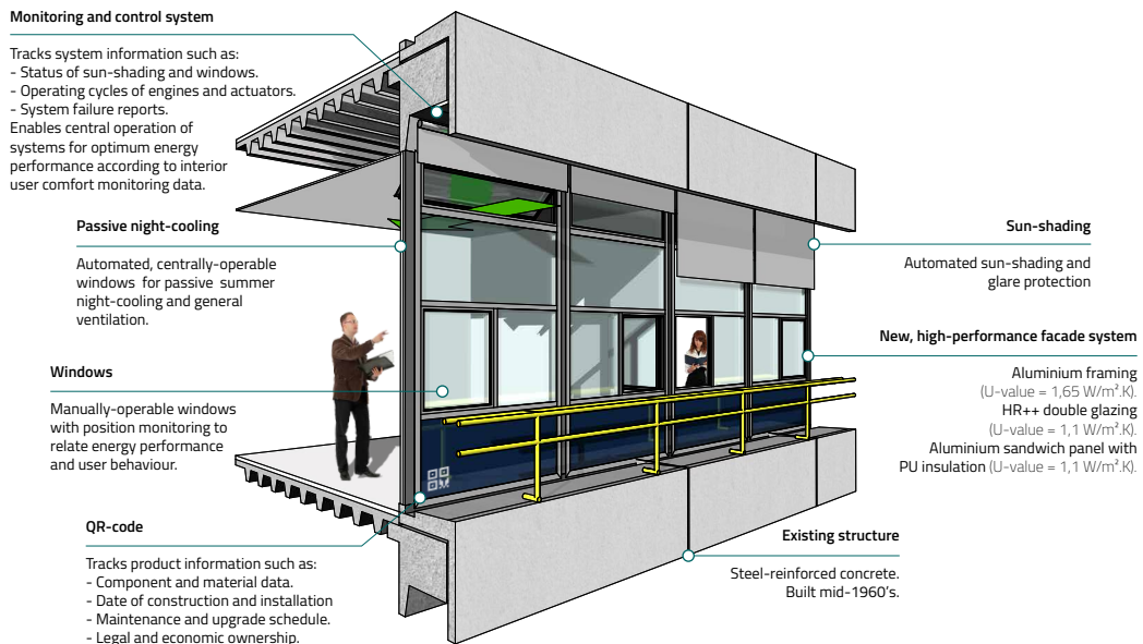
FIG. 3.9 Rendering of new CiTG Facade Leasing renovation solution, which includes high performance framing and glazing, centrally operable windows including an upper window for night-cooling airflow, and external solar shading with high-wind velocity resistance. The panels have also been designed in consultation with the original building architect to ensure its close resemblance to the original architectural appearance of the building.
