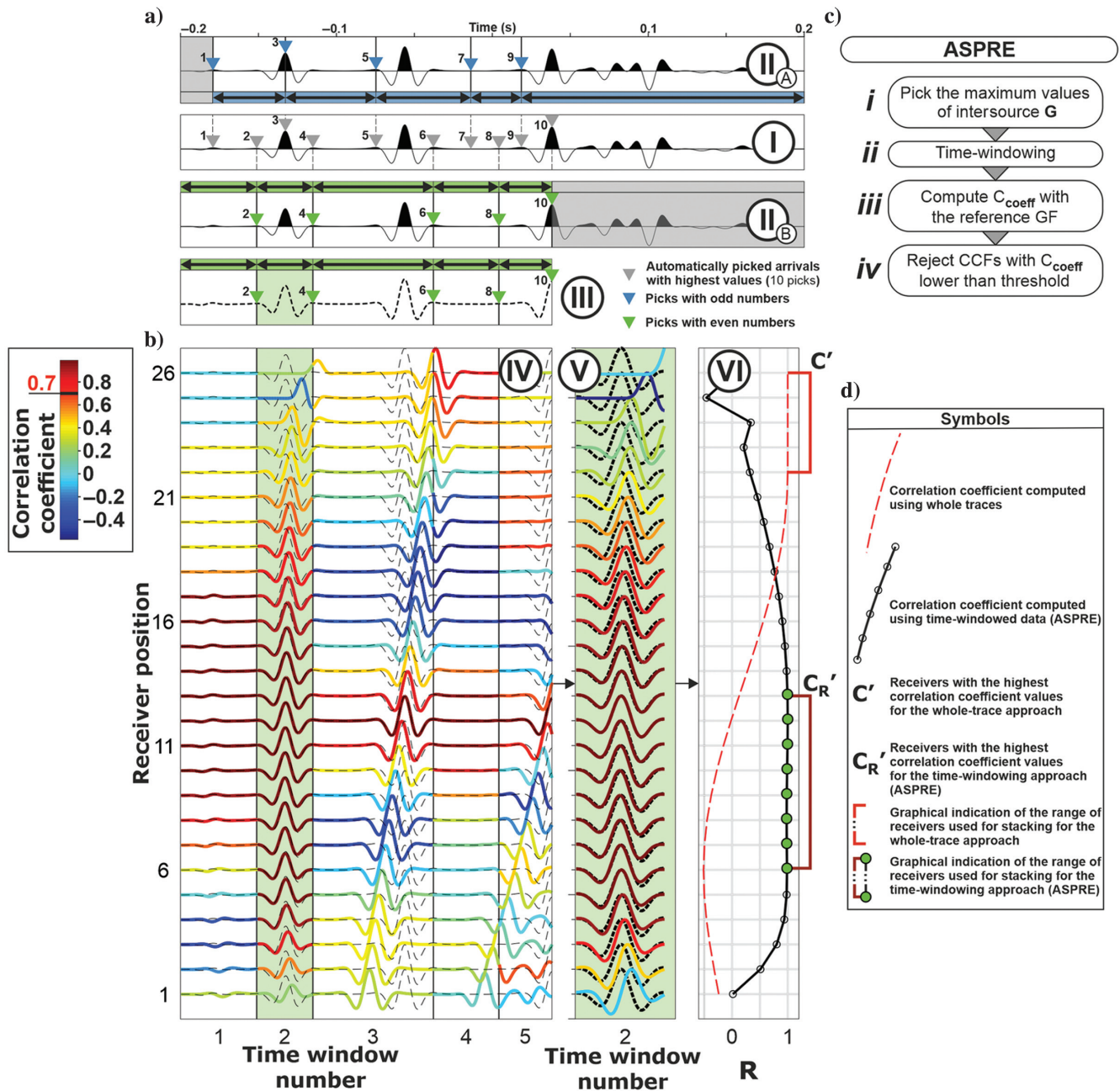
Figure 9. (a) Green’s function estimate from stacking all available receivers is shown in the panel I (same as Figure 8a, trace G). The gray triangles numbered 1–10 indicate selected positive peaks left and right of the reference positive peak at roughly -0.06 s. Panels II A and II B show the same trace G as in panel I, but with different time windows created based on the odd (1, 3, 5, 7, and 9) and even (2, 4, 6, 8, and 10) peaks, respectively. Horizontal arrows within the blue and green-shaded regions in panels II A and II B , respectively, show the size of the created time windows. Panel III shows the trace G divided into the windows that will be used for comparison with the correlation panel. Note that the trace is shown as a dashed line. The green-shaded window contains a reflection of interest. (b) Panel IV shows the correlation panel (colored lines) from Figure 8b with a superimposed trace from panel III (dashed black line). The color represents the CC value between the two traces in each window (see color-scale bar). Panel V shows a magnified version of the window of interest (window 2 in panel IV) where the phase shift at traces 1–3 and 24–26 is more easily visible. Panel VI shows the CC computed for window 2 in panels IV and V (black line), while also showing the CC values computed with the whole-trace approach (dashed red line). The stacking contours C'_R and C_R referred to in the text also are shown. (c) Detailed workflow of ASPRE. (d) Symbols used in (b).
