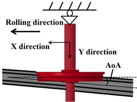
Fig. 7.8 Wheel-rail interaction model and the boundary conditions.
