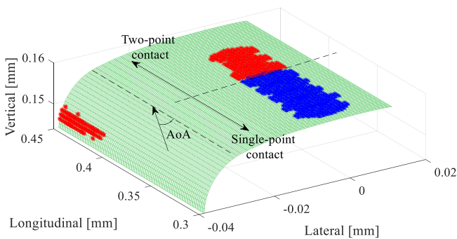
Fig. 7.9 Contact patches “footprints” (blue (dark gray in print version) for single-point contact and red (light gray in print version) for two-point contact).
