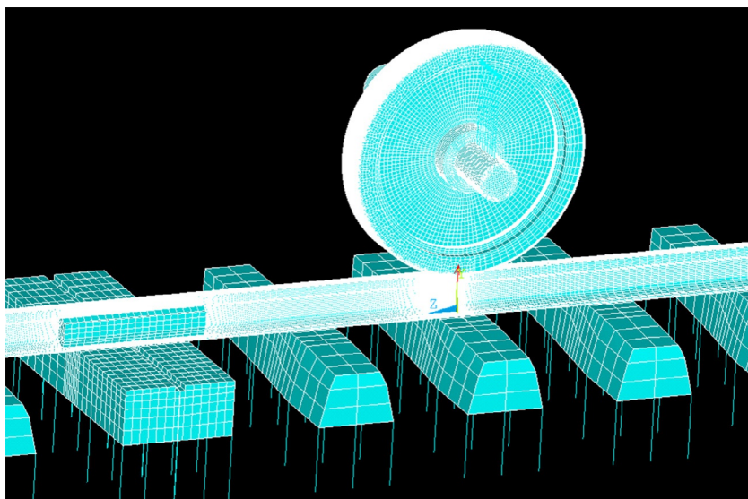
Fig. 7.2 A finite element wheel-IRJ dynamic interaction model.
