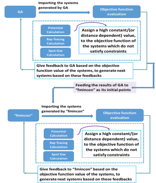
Fig.6. Schematic of optimization implementation for combined “fmincon” and GA.
