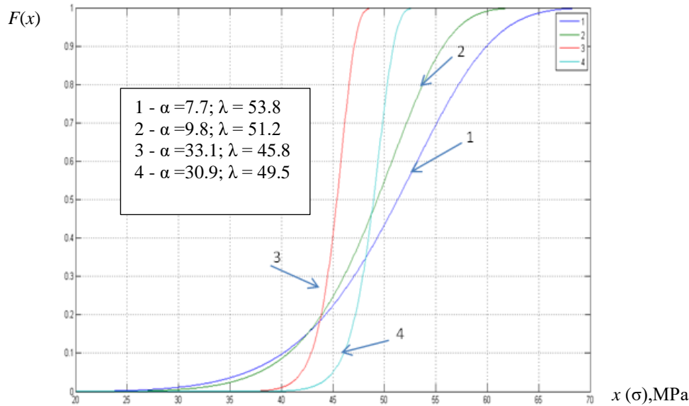
Fig.7 The Weibull distribution function F(x) for the form parameter \alpha and the scale parameter \lambda determined from equations (3) - (6): (3) - curve 1; (4) - curve 2; (5) - curve 3, (6) - curve 4
