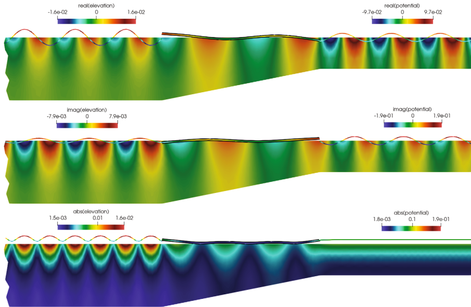
FIGURE 21 Close-up view of the velocity potential, \phi_h , and surface elevation, \eta_h , for the case \omega = 0.8 . Real part (top), imaginary part (center), and absolute values (bottom). The vertical direction of the domain is scaled 4:1 and the surface elevation is scaled by 1000. The beam region is shadowed in black.
