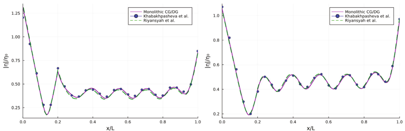
FIGURE 11 Relative surface elevation at the beam for the hinged case, \xi = 0 , (left) and the stiff joint, \xi = 625 , (right).
