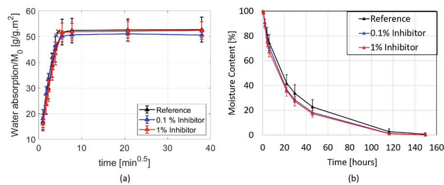
Fig. 4. (a) Capillary absorption (b) Drying behaviour of specimens with different inhibitor concentration.
