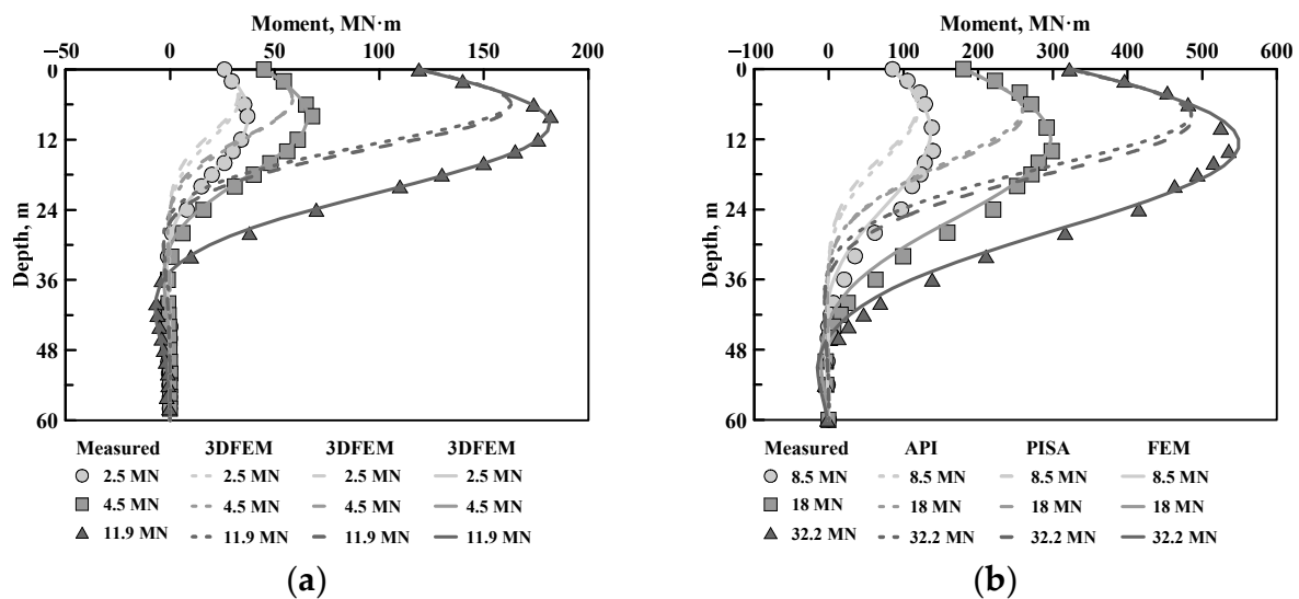
Figure 5. Comparison of measure and computed bending moment profiles of centrifuge tests: (a) D = 4 m, (b) D = 6 m.
