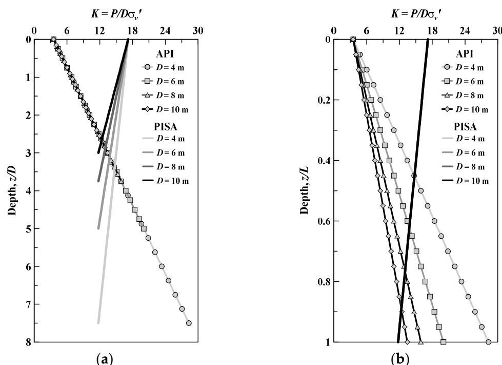
Figure 2. Normalized ultimate soil resistance profile against: (a) z/D , (b) z/L .
