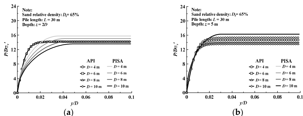
Figure 1. Typical p - y curves of API [21] and Burd et al. [25] at: (a) z = 2D , (b) z = 5 m.
