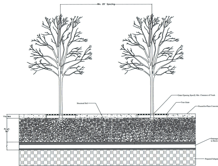
TYPICAL STREET TREE PLANTING - VIEW 2
