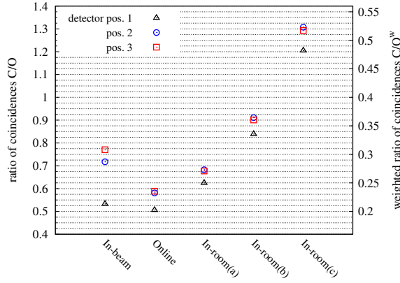
Figure 2.11: Carbon-to-oxygen (C/O) coincidence ratios in PMMA (modeled according to section 2.2.5), for different detector positions (figure 2.1-bottom) and acquisition protocols (figure 2.9). The carbon coincidences include contributions from ^{11}\text{C} and ^{10}\text{C} . The right axis displays the ratio of coincidences weighted by relative abundance of target nuclides ( \text{C/O}^w ).
