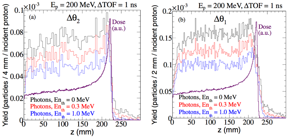
Figure 3.6: Prompt gamma profiles obtained with a proton energy of 200 MeV and the shifting TOF window indicated in figure 3.3(b), upon application of an energy threshold of 0.3 (red), 1.0 MeV (blue), or no threshold (black). Results are shown for both (a) the narrow angular collimation window \Delta\theta_2 and (b) the wide collimation window \Delta\theta_1 . All results were simulated with Geant4.
