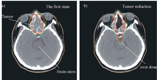
Figure 1.3: Example of a proton dose distribution for a tumor of the paranasal sinuses. Left : dose distribution at the beginning of the treatment. Right : dose distribution after several fractions. The reduction of the tumor volume gives rise to harmful overdosing of the radiation-sensitive brainstem. From (Nishio et al 2006).
