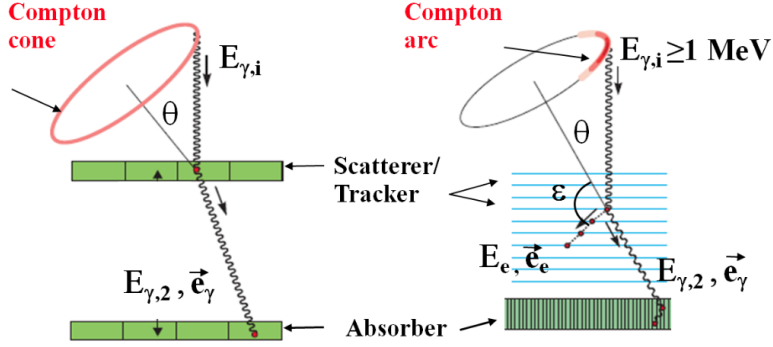
Figure 1.8: Illustration of the concepts of a single-layer 'γ-tracking' Compton camera (left) and an electron-tracking Compton camera (right). In γ-tracking mode, the position of Compton interaction and energy of the Compton electron ( E_e ) are detected in the scatterer, and both the (full) energy ( E_{\gamma,2} ) and the position of the scattered γ-ray are detected in the absorber, allowing for the determination of the direction of the scattered γ-ray ( \vec{e}_{\gamma} ), the initial γ-ray energy ( E_{\gamma,i} ) and the scattering angle \theta . In electron-tracking mode also the direction of incidence of the initial γ-ray can be determined to some extent, using the additional information of the electron trajectory ( \vec{e}_e ) obtained by means of a scatterer made of multiple thin layers. From (Thirolf 2015).
