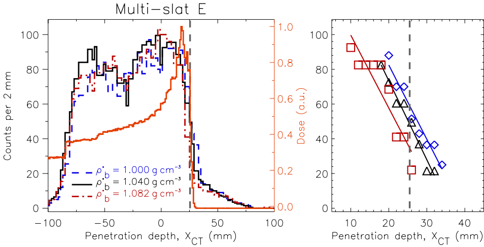
Figure 6.13: Left: Collimated prompt gamma profiles simulated for the irradiation of the NCAT pituitary region (figure 6.12), using multi-slat collimator E. Also shown is the laterally-integrated depth-dose profile in the case of original brain density ( \rho_b^* = 1.040 \text{ g cm}^{-3} ). A low-energy threshold of 1 MeV and a TOF acceptance window of 1 ns were applied, together with a median filter with a span of 8 bins (bin size = 2 mm). Right: data points in the distal falloff region of each profile, between the 20% and the 80% of each profile maximum, for over-dense (red squares), normal (black triangles), and hypo-dense brain tissue (blue diamonds), together with the corresponding linear regression fits. The vertical dashed lines in both graphs indicate the proton range in the case of the original brain density.
