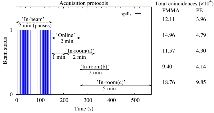
Figure 2.9: Definitions of acquisition protocols (left) and the corresponding measured total numbers of coincidences, post energy selection (displayed in-line on the right), from PMMA and PE phantoms. The coincidence counts were obtained with the detector placed at position 1 (figure 2.1-bottom). The 'in-beam' PET protocol corresponds to acquisitions during the beam pauses in between spills.
