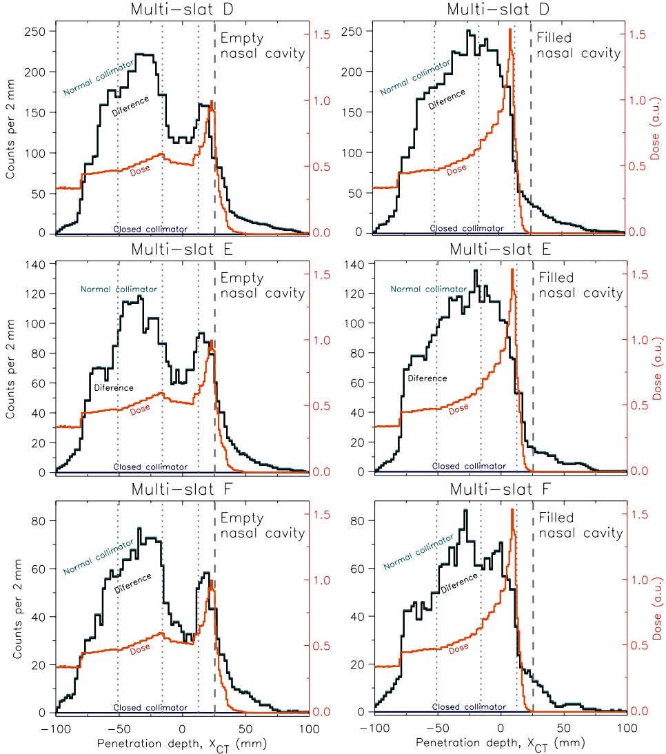
Figure 6.11: Collimated prompt gamma profiles simulated for the irradiation of the NCAT sphenoid region (figure 6.7), using the multi-slat collimators D-F (‘normal collimator’). Also shown are the laterally-integrated depth-dose profiles, the profiles from a closed collimator, and the ‘normal collimator’ profile after subtraction of the ‘closed collimator’ profile (‘diference’). A low-energy threshold of 1 MeV and a TOF acceptance window of 1 ns were applied, together with a median filter with a span of 12, 8, or 6 bins, for multi-slat collimators D, E, and F, respectively (bin size = 2 mm). The vertical dashed lines correspond to the proton range in the planned, ‘Empty nasal cavity’ situation. The vertical dotted lines represent soft-tissue/bone, bone/nasal-cavity, and nasal-cavity/bone interfaces traversed by the protons, from left to right, respectively.
