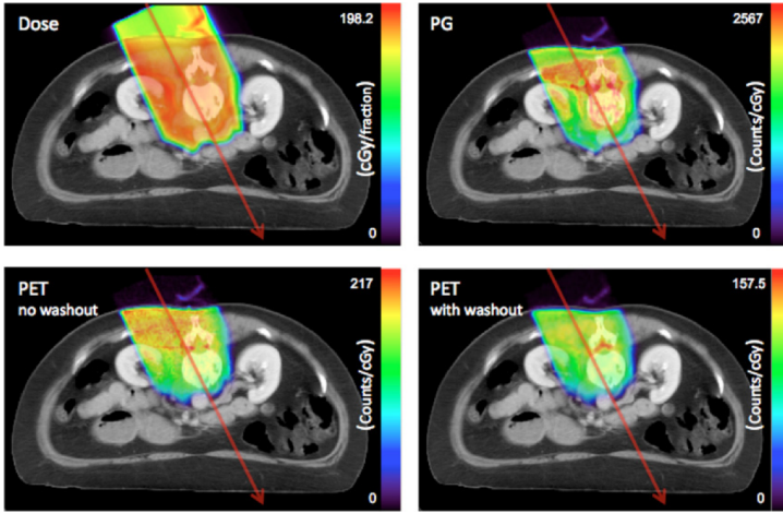
Figure 1.9: Geant4 simulation corresponding to a proton treatment in the dorsal region. The top-left image shows the dose distribution of the treatment, whereas the top-right one depicts the location of PG creation originated by the same treatment. The two bottom images correspond to the distribution of created \beta^+ emitters without (left) and with (right) biological washout for a measuring time complying to an in-room PET solution. From (Moteabbed et al 2011).
