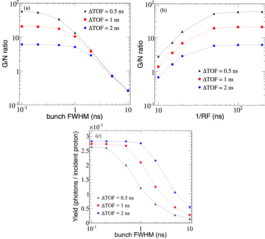
Figure 3.8: Gamma-to-neutron ratio (G/N ratio, see the text for explanation) as a function of (a) the proton bunch width (bunch FWHM) and (b) the accelerator repetition period ( 1/\text{RF} ), as well as (c) the number of photons detected as a function of the bunch width, for TOF windows \Delta\text{TOF}_z of 0.5 (black triangles), 1.0 (red squares) and 2.0 ns (blue circles). All calculations were performed for a proton energy of 200 MeV and are averaged over the detector region 0 \leq z \leq R .
