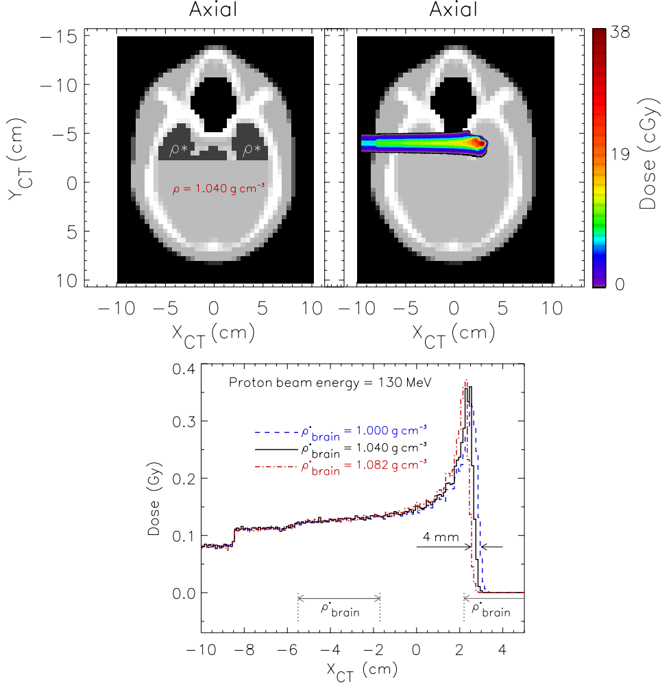
Figure 6.12: Top-left: NCAT-head axial slice showing the region in dark-grey color where the brain density was changed ( \rho^* ) by \pm 4\% relative to the original value ( \rho = 1.040 \text{ g cm}^{-3} ). Top-right: Dose distribution corresponding to 130 MeV proton irradiation of the pituitary gland (original brain density). Bottom: depth-dose profiles in the center of the pencil beam for the three brain-density cases studied.
