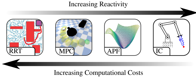
Figure 3.1: Reactivity scale of different motion planning methods revised in this thesis. Global methods, such as Rapidly-exploring Random Tree (RRT) [29] are at the least reactive end. More reactive methods, such as Model Predictive Control (MPC) [7], Artificial Potential Fields (APF) [30] and low-level control methods such as Impedance Control (IC) [12] are towards the more reactive side.
