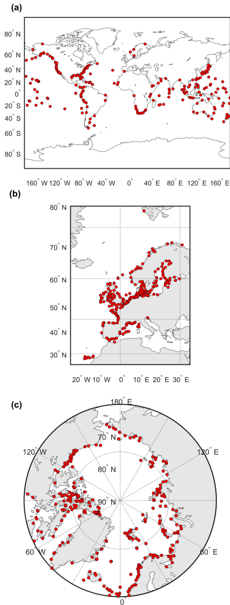
Figure 1.3: Available tide gauge locations (a) UHSLC dataset; (b) CMEMS dataset; (c) Arctic stations.
