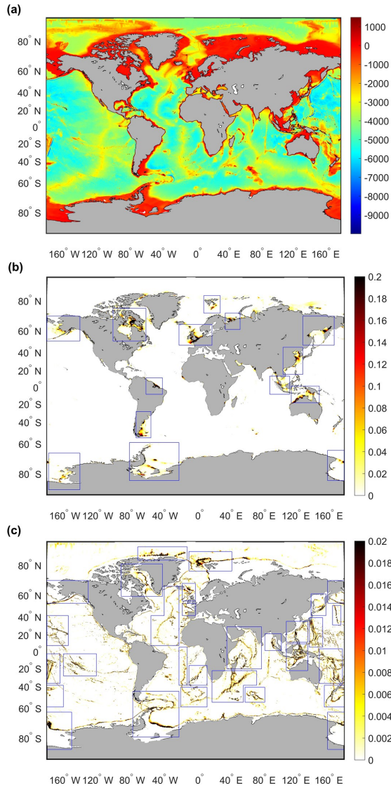
Figure 2.1: Spatial distribution of uncertain parameters. (a): Bathymetry [m]; (b): Tide energy dissipation by bottom friction in [\text{W/m}^2] ; (c): Tide energy dissipation by internal tides friction. The areas with large tidal energy dissipation are shown in the areas with blue boxes.
