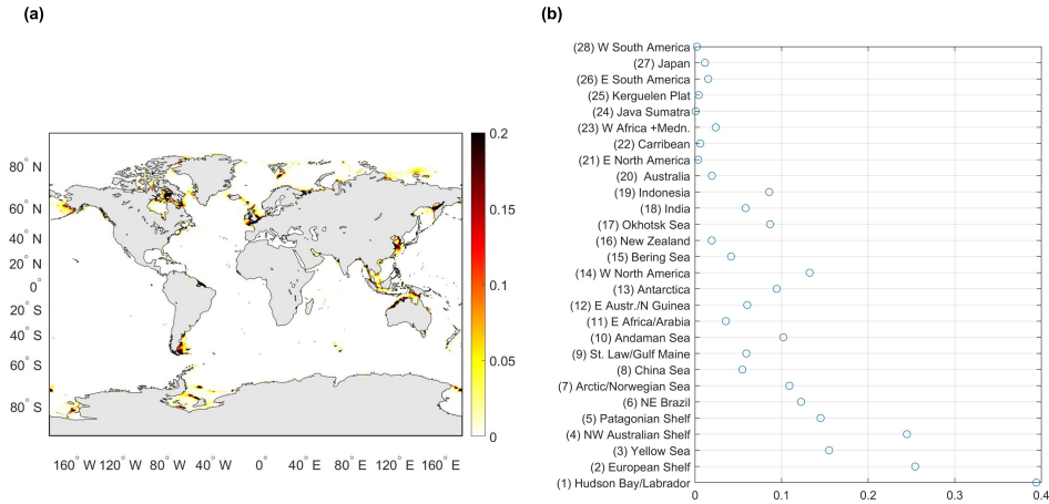
Figure 5.1: Bottom friction energy dissipation in initial GTSMv4.1 (a) Global distribution [Unit: W/m^2 ]; (b) Area-integrated energy dissipation [Unit: TW ].
