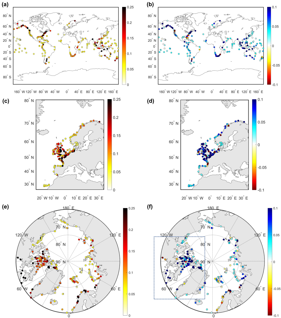
Figure 5.2: Left column: RSS between initial GTSMv4.1 and tide gauge data. Right column: RSS difference between initial GTSMv4.1 and FES2014 dataset (RSS of GTSM minus RSS of FES2014). Color blue shows better performance in FES2014 than GTSM. (a),(b) UHSLC dataset; (c),(d) CMEMS dataset; (e),(f) Arctic stations.[unit: m]
