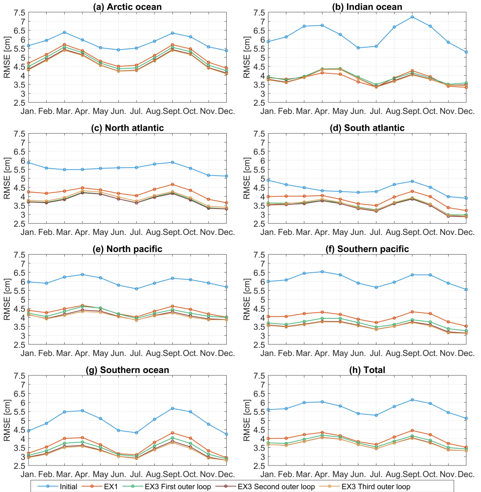
Figure 4.9: RMSE between model output and FES2014 dataset in 2014.
