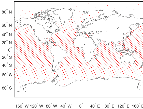
Figure 3.1: Observation locations: 1973 time series from the FES2014 dataset.
