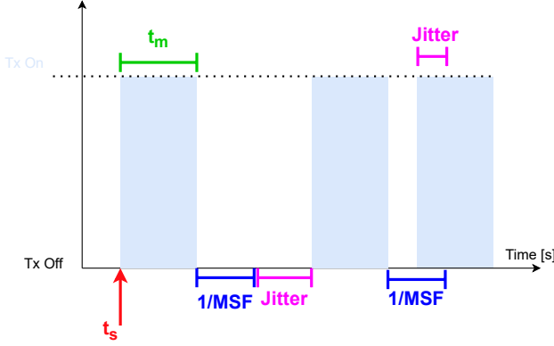
Fig. 5. Model of the timing for the message transmission with jitters (not to scale)
