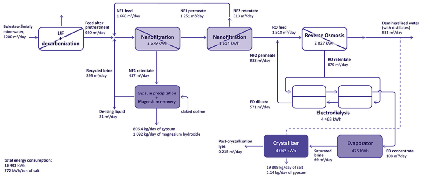
Fig. 7. Schematic overview of pre-treatment and concentration phases.
