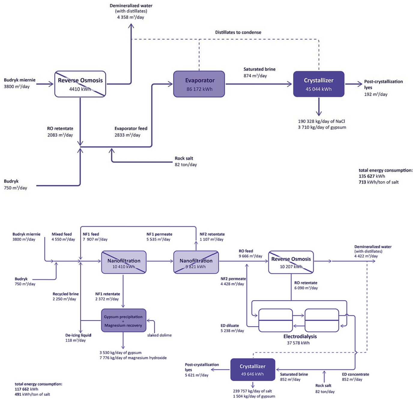
Fig. 3. Design of Dębniński wastewater treatment plant (top drawing) and ZERO BRINE design for Debiensko wastewater treatment plant (bottom drawing).
