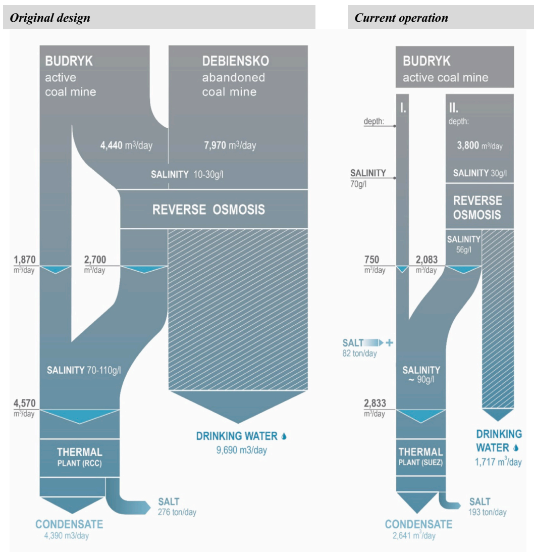
Fig. 2. Material balance of Dębniński case (left picture: original design, right picture: current operation).
