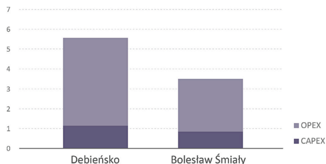
Fig. 11. Unit cost per cubic meter treated for the coal mine effluents generated by Debieńsko and Bolesław Śmiały coal mines.
