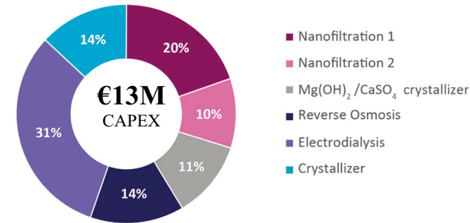
Fig. 4. Capital expenditure (CAPEX) for improved Dębieńsko desalination plant.
