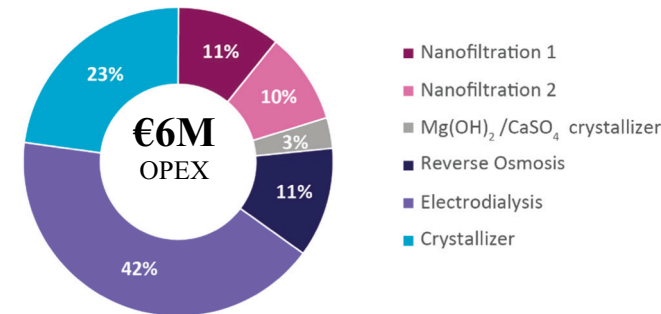
Fig. 5. Annual operating expenditure (OPEX) for improved Dębieńsko desalination plant.
