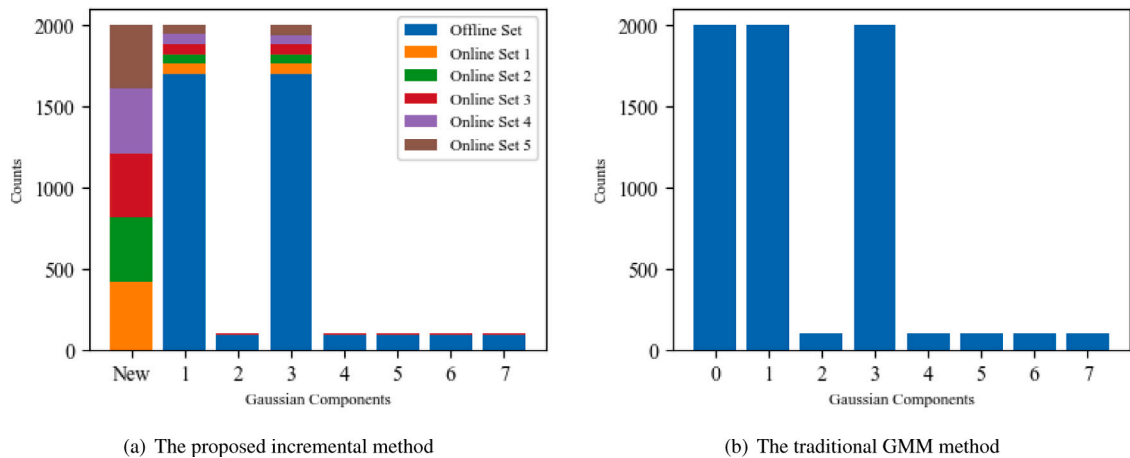
Fig. 13. Number of data in each cluster by the proposed incremental method and the traditional GMM in Simulation Data I.
