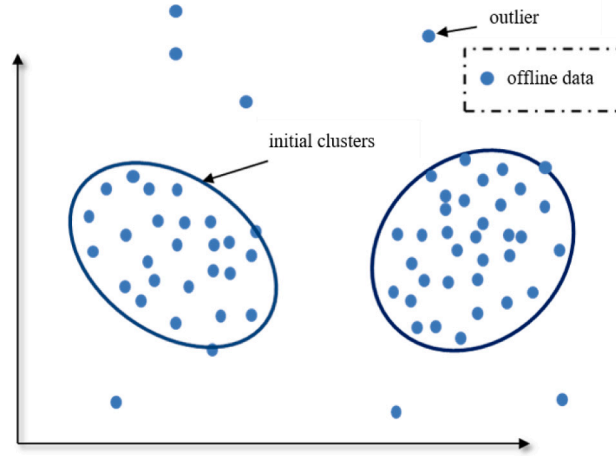
Fig. 4. Initial GMM.
