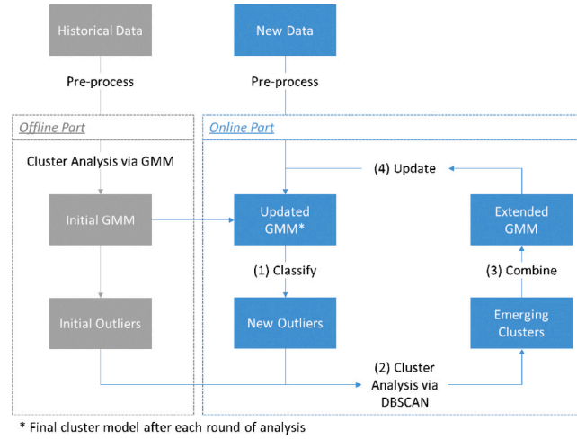
Fig. 3. An Incremental Clustering Method for Anomaly Detection in Flight Data.
