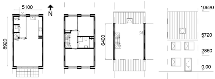
FIGURE 3.3 Plans and sections of the Dutch reference row house
