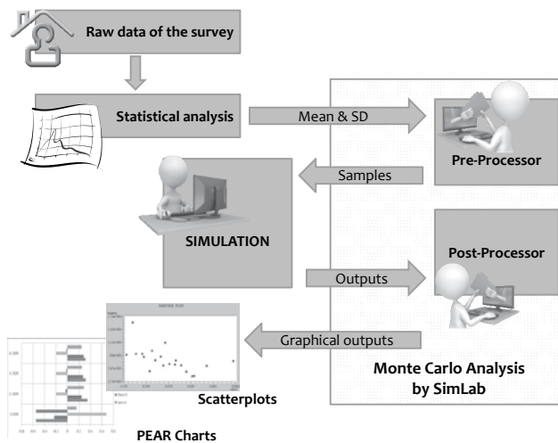
FIGURE 3.2 Flow chart of the study methodology
