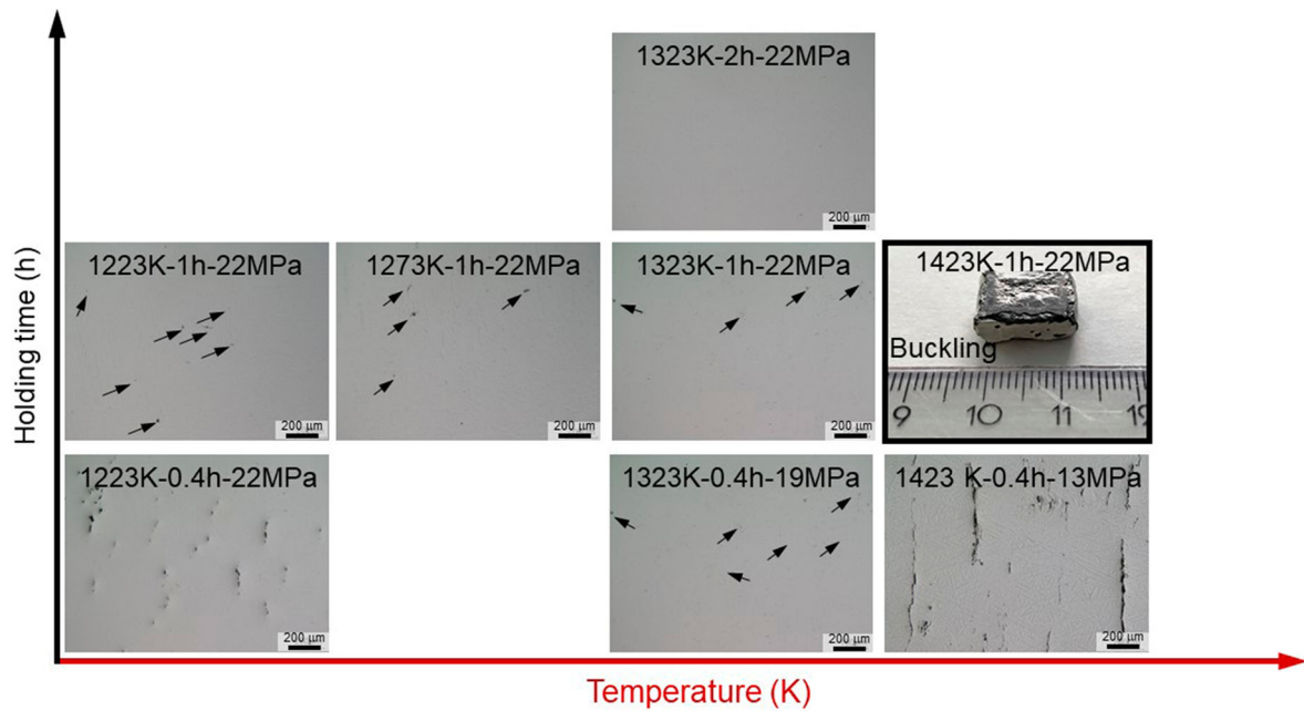
Figure S1. Optical microstructure of NiTi processed by various SPS parameters (shown in the figure in the format of 'Temperature (K)-Holding time (h)-Pressure (MPa)'). All images are with 200 μm scale bars. Micro-cracks are marked by black arrows in the figure.
