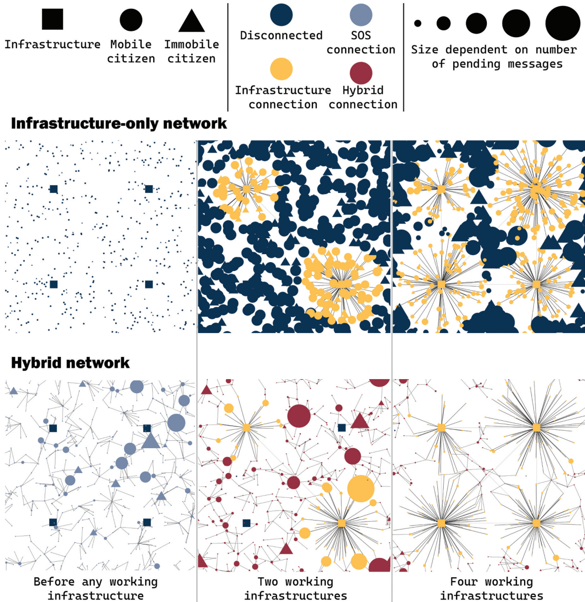
Figure 4. Screenshots of the infrastructure-only and hybrid networks simulations are presented for three instances. Mobile citizens are circles; triangles represent immobile citizens. Infrastructure equipment is square. In the top rows, the infrastructure-only network is displayed. In the bottom row, the hybrid network simulation is displayed. In each row, screenshots corresponding to three different moments are displayed. First, when no infrastructure is available, the hybrid network relies solely on the SOS ad hoc mobile network (in sky blue). In the second screenshot, two infrastructures are active. For infrastructure-only, phones in the coverage area of the two infrastructures are connected (in yellow). For the hybrid network, phones in the range of infrastructure are directly connected (in yellow), other phones are indirectly linked to the infrastructure in hybrid mode (in red), and a few are in SOS mode (in sky-blue). In the last screenshot, all four infrastructures are active.
