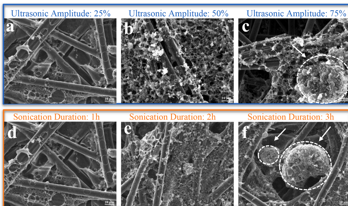
Fig. 6. Effects of different ultrasonic treatments on the surface morphology of the PVF/CNT electrodes obtained treated by electrochemical oxidation. Scanning electron microscopy (SEM) images of the electrodes exposed for (a) 25 %, (b) 50 %, (c) 75 % ultrasonic amplitude at PVF/CNT 1 and 1-h ultrasonic time; (d) 1 h, (e) 2 h, (f) 3 h ultrasonic time at PVF/CNT 1 and 25 % ultrasonic amplitude.
