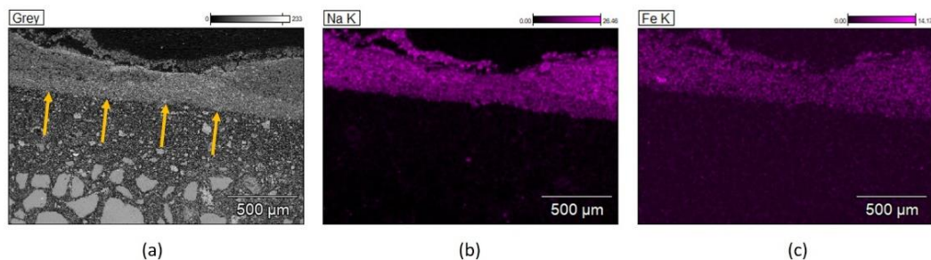
Figure 1: SEM-EDS map of the top 2mm of a polished section of a mortar specimen at the end of 1st wet-dry cycle. (a) Accumulation of NaFeCN crystals near the surface due to capillary transport confirmed by elemental mapping of (b) Na and (c) Fe
