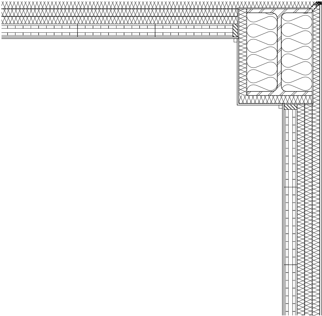
Corner connection
