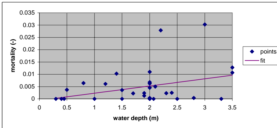
Figure 2.3 Proposed function for flood mortality estimation due to other causes
