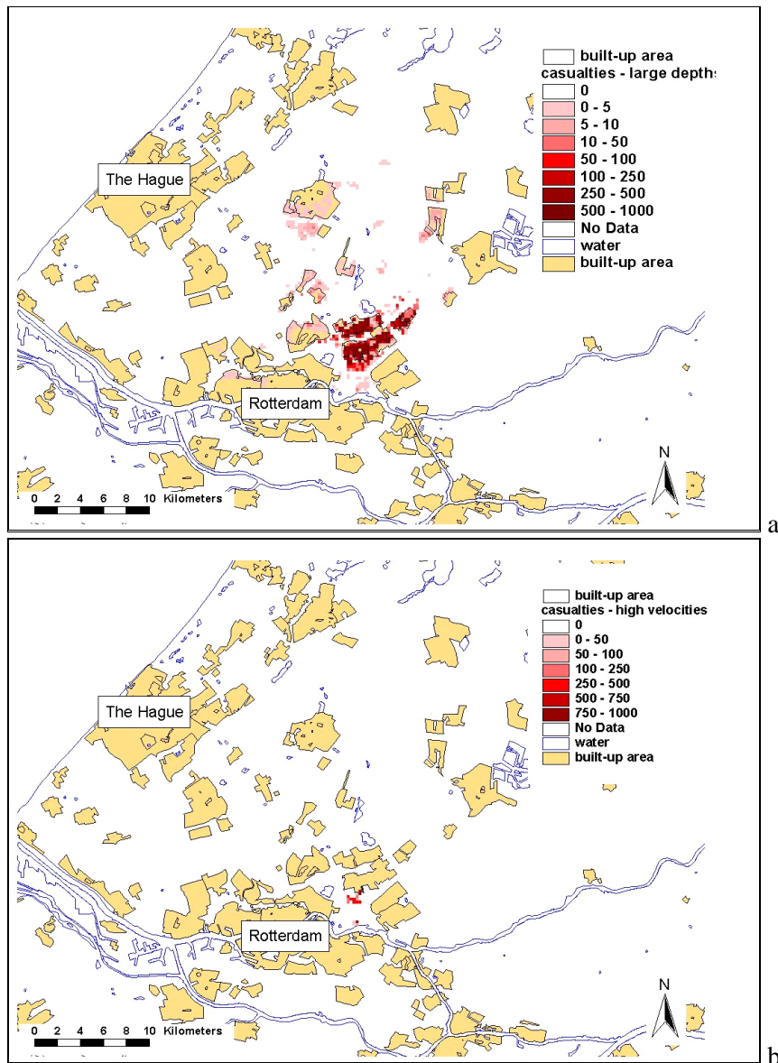
Figure 5.4 Estimated number of fatalities per grid cell of 250x250 m 2 when the required time for evacuation is 50 hours: (a) fatalities caused by large water depths, (b) fatalities caused by high flow velocities
