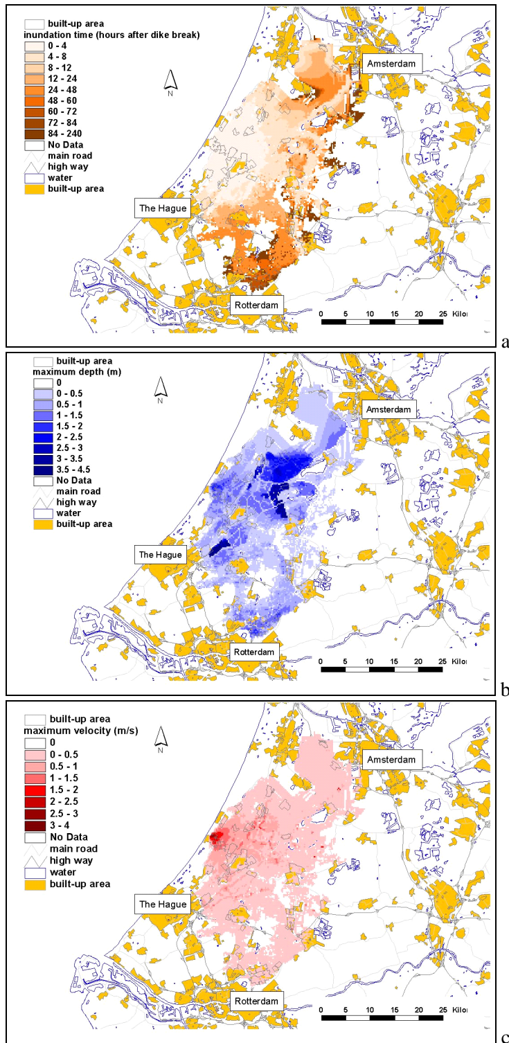
Figure 5.5 Flood characteristics computed with the 2D hydraulic model: (a) time of inundation (hours after failure of the river dike), (b) maximum water depth (m), (c) maximum flow velocity (m/s)
