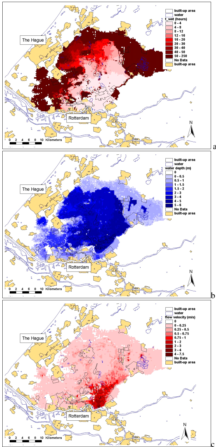
Figure 5.2 Flood characteristics computed with the 2D hydraulic model: (a) time of inundation (hours after failure of the river dike), (b) maximum water depth (m), (c) maximum flow velocity (m/s)
