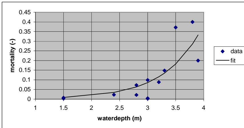
Figure 2.1 Proposed function for estimation of flood mortality for rapidly rising water
