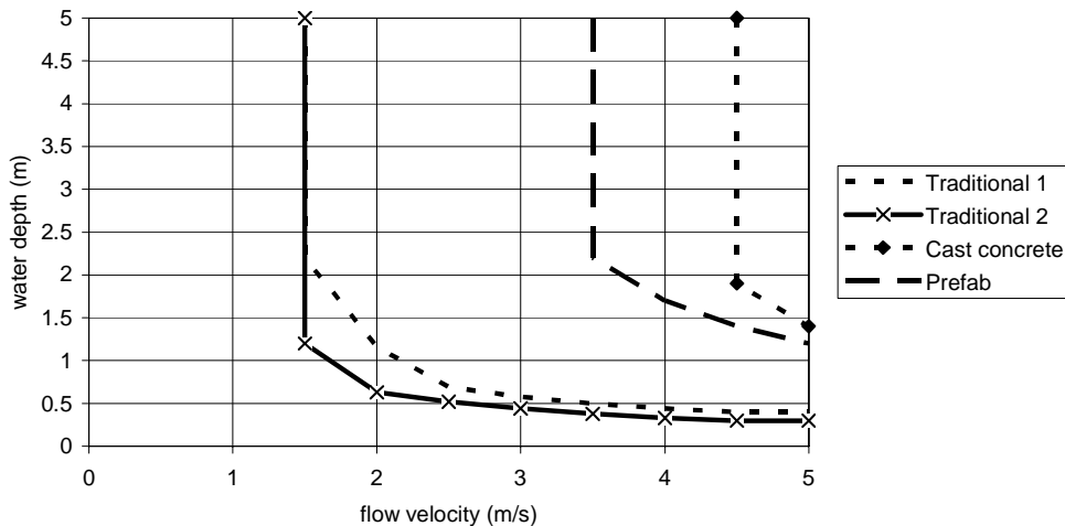
Figure 2.3 Combination of flow velocity and water depth for which a wall of a certain type of building stock will collapse with 100% probability, based on Roos et al (2003)
