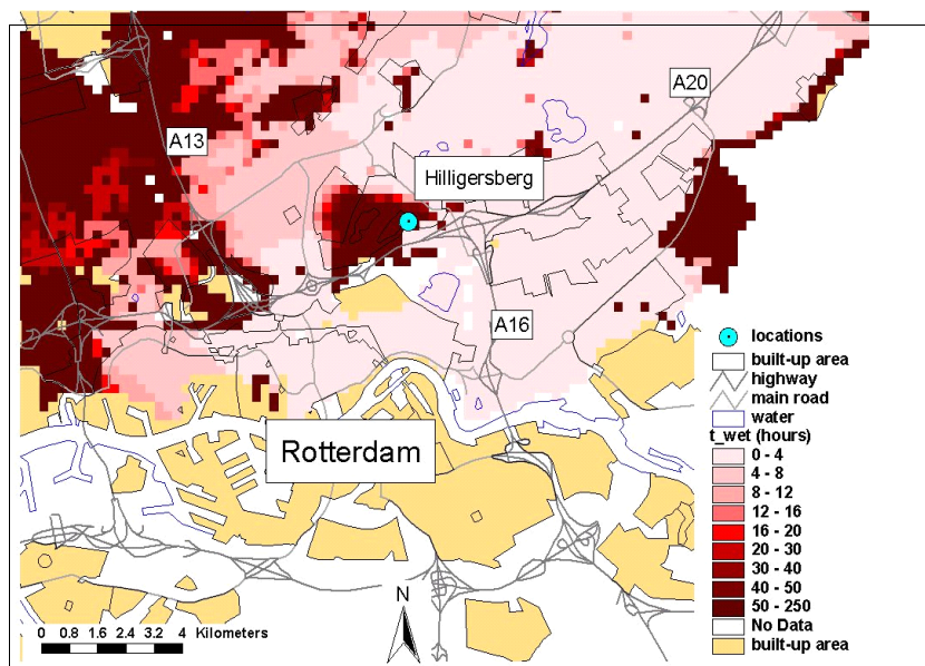
Figure 5.8 Detailed map of time of inundation near Rotterdam Hilligersberg
