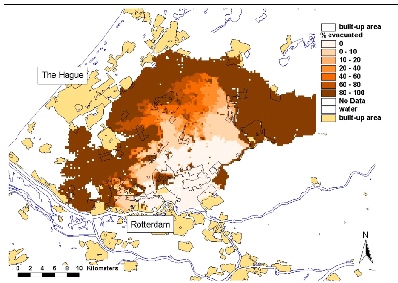
Figure 5.3 Percentage of inhabitants that can evacuate or escape when the total time required for evacuation equals 50 hours
