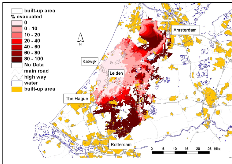
Figure 5.6 Percentage of inhabitants that can evacuate or escape when the total time required for evacuation equals 50 hours
