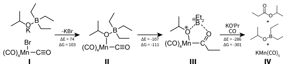
Figure 4.11. Proposed reaction mechanism for the Mn-mediated alkoxy carbonylation of organoboranes. DFT calculations were performed at the PBE0-D3(BJ)-SMD(THF)/6-311+g(d,p) level of theory at 298.15 K in THF. \Delta E and \Delta G represent the reaction energy and Gibbs free energy changes in \text{kJ mol}^{-1} .
