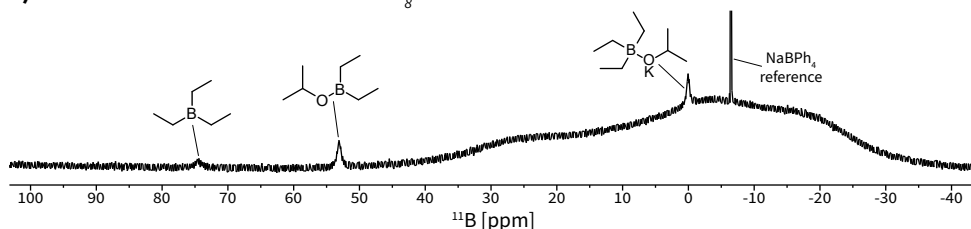
Figure 4.12. Spectroscopic support for the proposed reaction mechanism. Conditions: Mn(CO) 5 Br + 1 eq. K[Et 3 B(O i Pr)] + 1 eq. KO i Pr in THF. Spectra were recorded after ~1 h at room temperature. a) Solution FTIR transmission spectrum after reaction in THF (~0.5 mg Mn ml -1 ). b) 1 H NMR spectrum after reaction in THF- d 8 (400 MHz). c) 11 B NMR spectrum after reaction in THF- d 8 (128 MHz).
