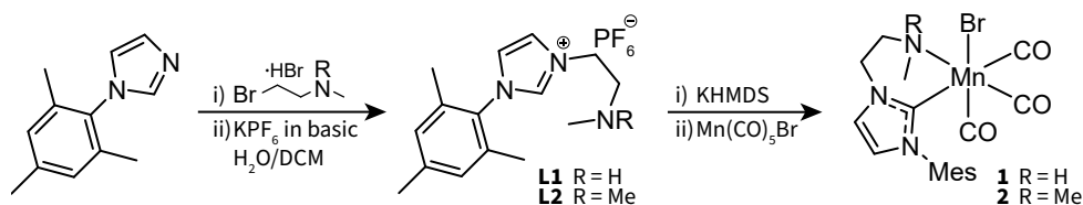
Figure 3.2. Synthetic route towards \text{Mn}^{\text{I}} -NHC complexes 1 and 2 .
