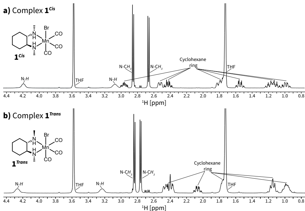
Figure 2.4. ^1\text{H} NMR spectra of Mn II -N,N' complexes in THF- d_6 (400 MHz). a) 1 cis . b) 1 trans .
