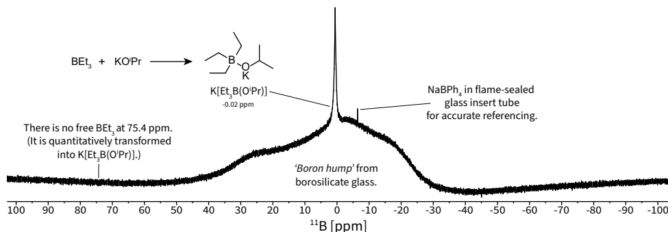
Figure 4.4. Formation of potassium triethyl(isopropoxy)borate and its corresponding ^{11}\text{B} NMR spectrum (128 MHz, \text{THF}-d_8 ).
