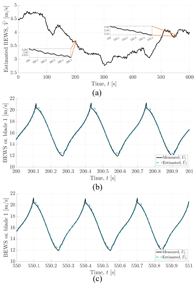
Fig. 7. Estimation results for a realistic turbulent wind profile with a mean wind speed of 4 m/s and a turbulence intensity of 20 %: (a) time traces of the estimated rotor-effective wind speed, (b) and (c) blade-effective wind speed for blade 1 for two different time frames.
