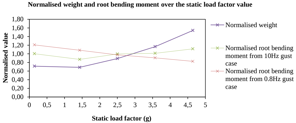
Figure 9: Summary of the weight and root bending moment of the different optimisation run.
