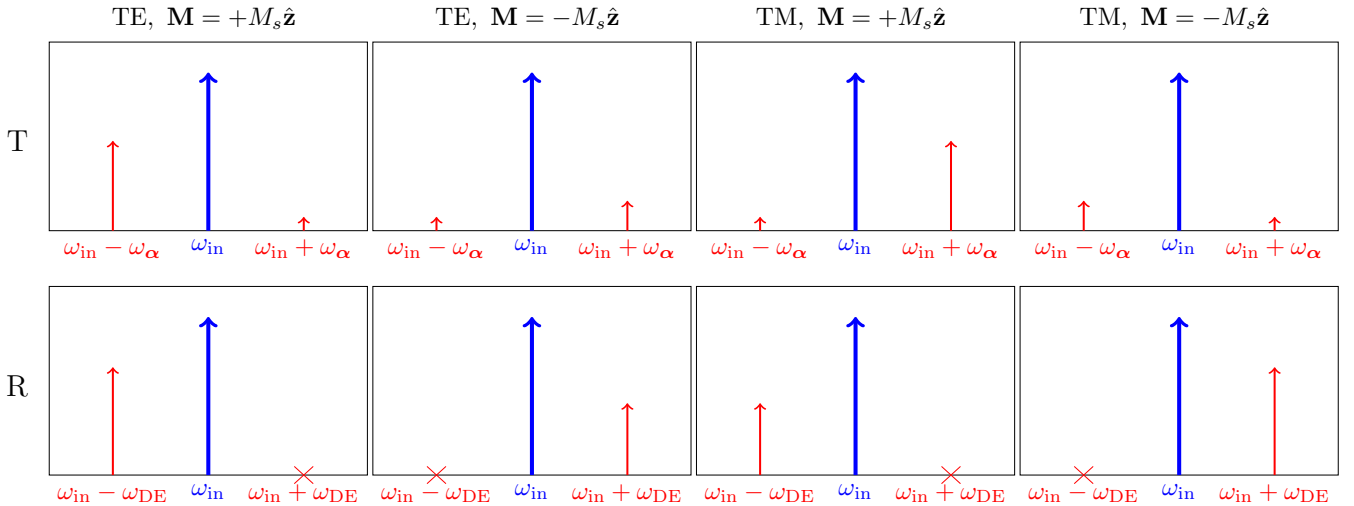
FIG. 7. Schematic light scattering spectra by a magnetic sphere in proximity to a single-mode optical fiber, emphasizing the S-aS asymmetry. The blue arrow marks the frequency \omega_{\text{in}} of light input and the panel T (R) denotes the transmission (reflection) spectra with Stokes and anti-Stokes lines. \omega_\alpha and \omega_{\text{DE}} are the resonance frequencies of magnons involved in the transmission and reflection, respectively. Each column corresponds to one of the four cases, \sigma \in \{\text{TE}, \text{TM}\} or \mathbf{M} \parallel \pm \hat{\mathbf{z}} . A cross denotes complete absence of a peak by chirality selection. The peak heights are not on scale, but peaks with the same height have power in the same order of magnitude. We assume that the input frequency and the magnetic field have been tuned to the resonant scattering condition in each case as discussed in the main text.
