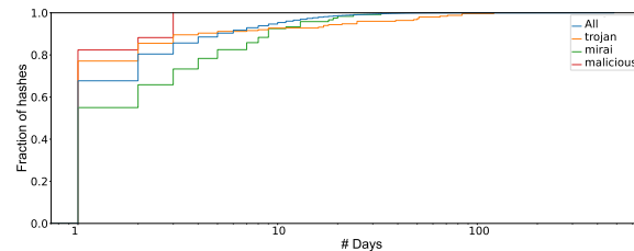
Figure 22: ECDF: length of attack campaigns by attack type.
