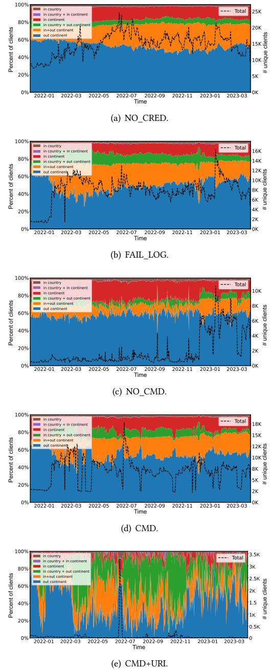
Figure 24: Regional diversity: client vs. honeypot by category.
