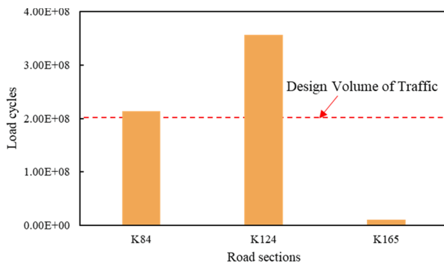
Fig. 16. The estimated residual life of the pavemen.
