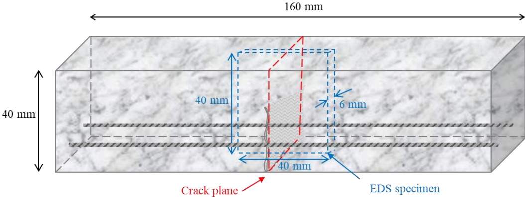
Figure 7.6 Location of specimen for EDS scanning in cracked mortar prism
