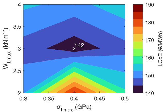
Figure 9. LCoE as a function of maximum wing loading W_{l,\text{max}} and maximum tether stress \sigma_{t,\text{max}} . The other design variables are held constant with the following values: wing area S = 60 \text{ m}^2 , aspect ratio \text{AR} = 12 , and power crest factor f_{\text{crest}} = 2 .
