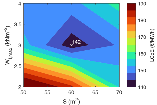
Figure 7. LCoE as a function of wing area S and maximum wing loading W_{l,\text{max}} . The other design variables are held constant with the following values: aspect ratio AR = 12 , maximum tether stress \sigma_{t,\text{max}} = 0.4 \text{ GPa} , and power crest factor f_{\text{crest}} = 2 .
