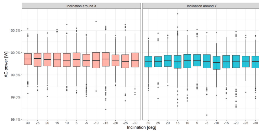
(a) Normalised delivered AC power during static test.
