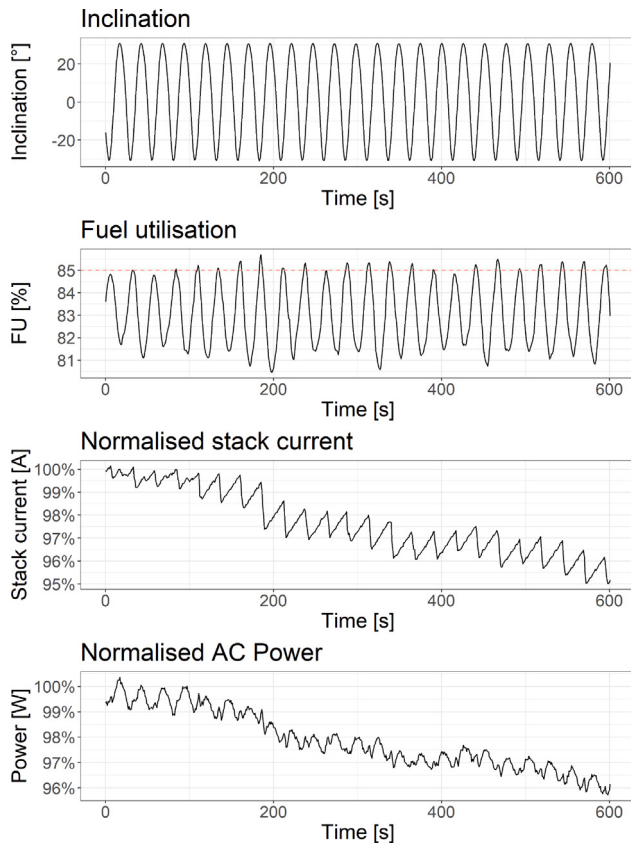
Fig. 4. Inclination, fuel utilisation, stack current and AC Power over testing time for the dynamic experiment using rotation around X-axis, an angle of 30 degrees and a period of 27 s. The stack current and AC power are given as a percentage of their nominal value.
