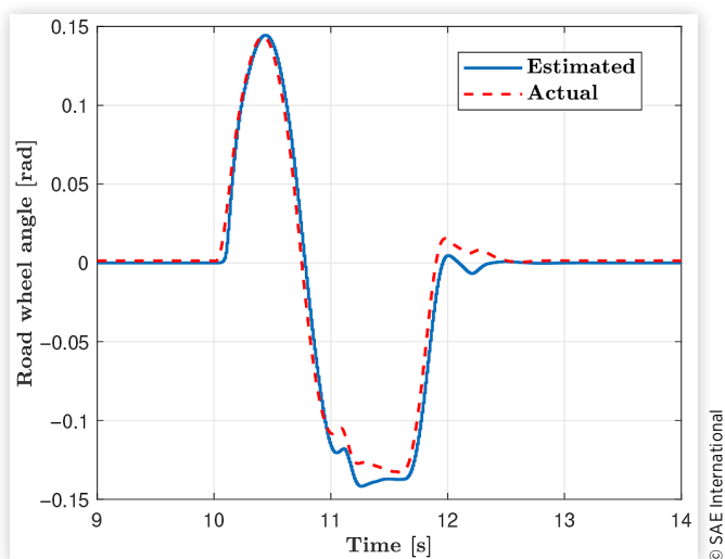
FIGURE 9 Road wheel angle—APE+MPCA.
