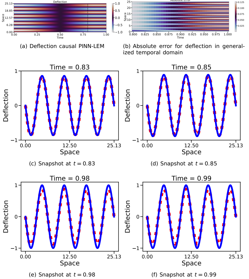
Figure 5.3: Euler-Bernoulli beam on the Winkler foundation: Various analyses and temporal snapshots.
