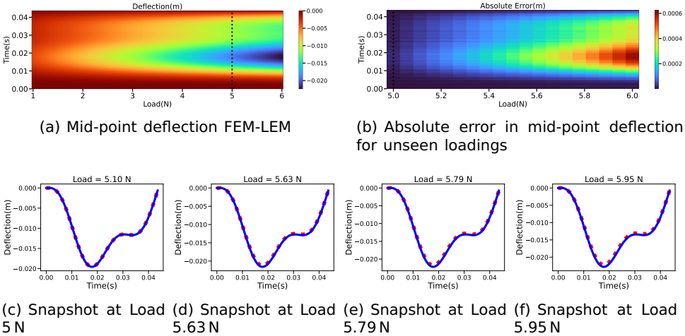
Figure 5.5: Mid-point deflection for Moving load: Analysis and load snapshots.
