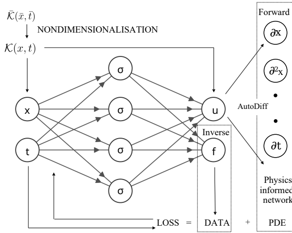
Figure 2.4: PINN framework for beam systems: For forward problems, the loss function comprises the nondimensional PDEs and the boundary and initial conditions. For inverse problems, the nondimensional PDEs are supplemented with extra data and potential initial/boundary conditions.
