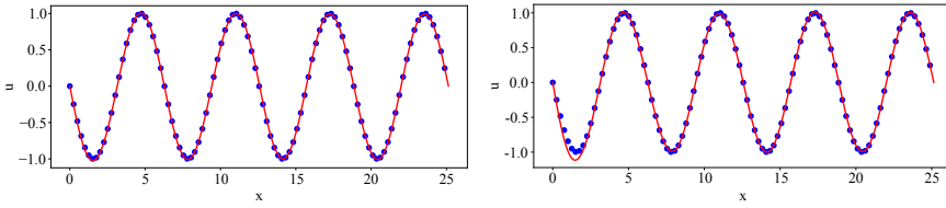
Figure 3.4: Euler-Bernoulli beam equation on the Winkler foundation with noise in the initial condition of displacement of the beam Left: Predicted solution at final time ( t = 1 ) with 10% Gaussian noise; Right: Predicted solution at final time ( t = 1 ) with 20% Gaussian noise. Blue dots are ground truth and red curve is prediction.
