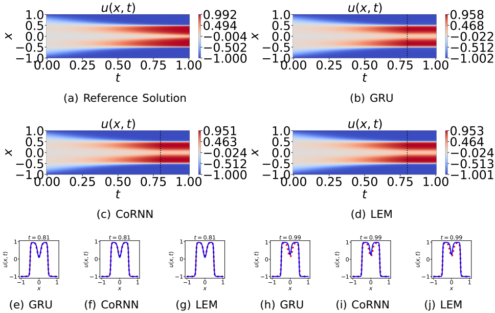
Figure 4.3: Top two rows: the complete reference solution and predictions for the Allen-Cahn equation. Bottom: the solution snapshots at t = \{0.81, 0.99\} obtained in the generalization region.
