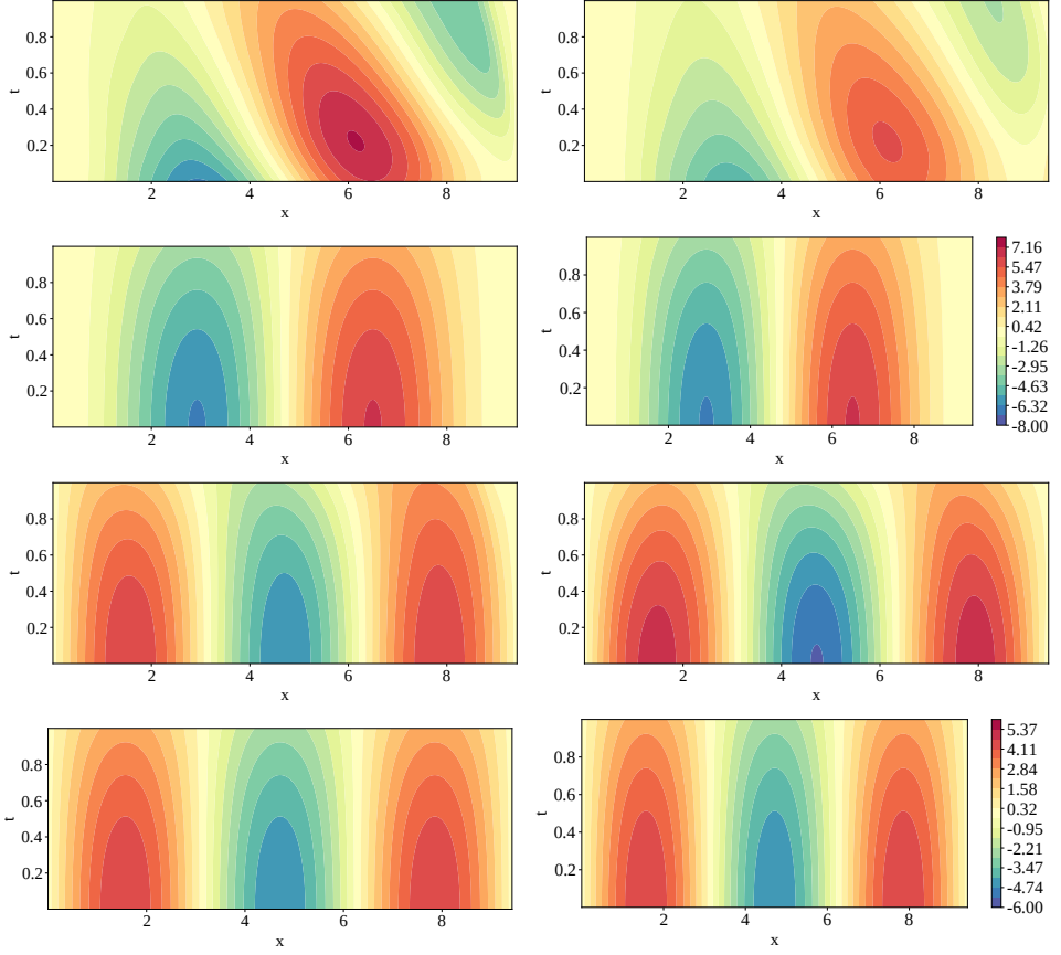
Figure 3.8: Timoshenko beam on the Winkler foundation First row: Predicted Displacement ( u^* ) ( Left. ) Using PINN ( Right. ) Using SA-PINN ( Second row, Left. ) Using causal PINN ( Right. ) Reference solution Third row: Predicted Rotation ( \theta^* ) ( Left. ) Using PINN ( Right. ) Using SA-PINN ( Fourth row, Left. ) Using causal PINN ( Right. ) Reference solution
