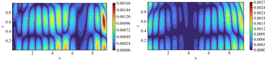
Figure 3.9: Timoshenko beam on the Winkler foundation at final time t = 1 . Left: Absolute error in predicting displacement ( |u - u^*| ); Right: Absolute error in predicting rotation ( |\theta - \theta^*| )
