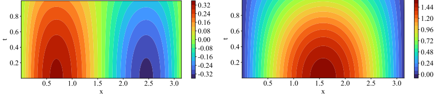
Figure 2.5: Timoshenko single beam; Color bar represents Left: Cross-sectional rotation ( \theta^* ); Right: Transverse displacement ( w^* ).
