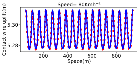
(c) Contact wire uplift prediction at 80 \text{ km h}^{-1}
