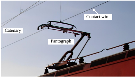
(a) Real-world catenary-pantograph setup in railways
