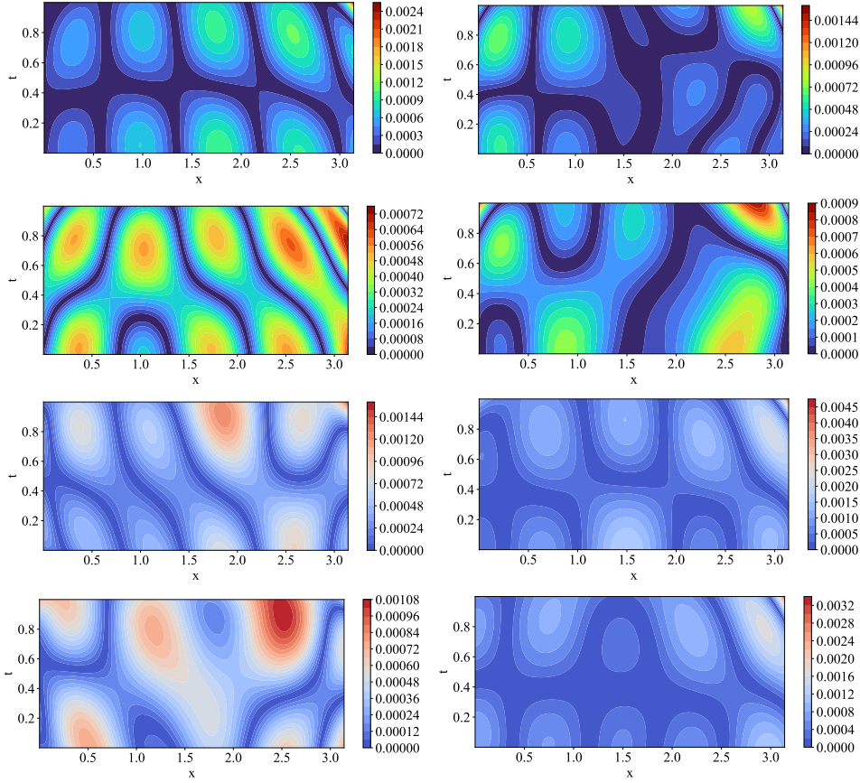
Figure 2.12: Timoshenko double beam absolute errors in prediction; \theta_1 and w_1 are the rotation and displacement of the first beam, \theta_2 and w_2 are the rotation and displacement of the second beam First row 16000 training points (Left) |\theta_1 - \theta_1^*| ; (Right) |w_1 - w_1^*| ; (Second row, Left) |\theta_2 - \theta_2^*| ; (Right) |w_2 - w_2^*| . Third row 1600 training points (Left) |\theta_1 - \theta_1^*| ; (Right) |w_1 - w_1^*| ; (Fourth row, Left) |\theta_2 - \theta_2^*| ; (Right) |w_2 - w_2^*| .
