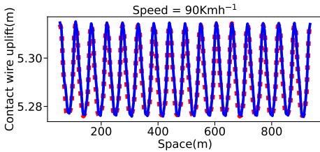
(e) Contact wire uplift prediction at 90 \text{ km h}^{-1}
