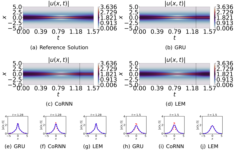
Figure 4.4: Top two rows: the complete reference solution and predictions for the Schrödinger equation. Bottom: the solution snapshots at t = \{1.28, 1.5\} obtained in the generalization region.
