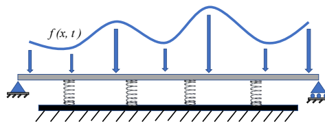
Figure 3.1: Simply supported beam on an elastic foundation under varying transverse force
