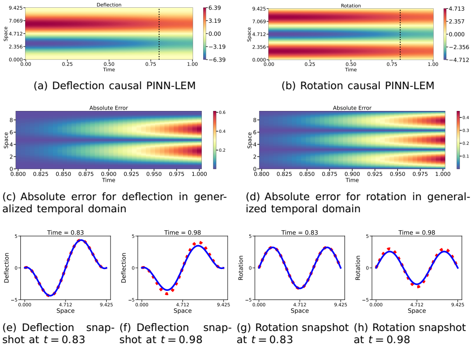
Figure 5.4: Timoshenko beam on the Winkler foundation: Detailed analysis and temporal snapshots.
