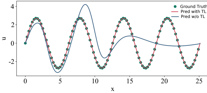
Figure 3.7: Euler-Bernoulli beam on the Winkler foundation for initial velocity for case 1: Causal PINN prediction at final time t = 1 with and without transfer learning
