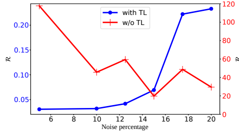
Figure 3.6: \mathcal{R} vs noise percentage in the initial condition for the Euler Bernoulli beam for both approaches - with and without transfer learning.
