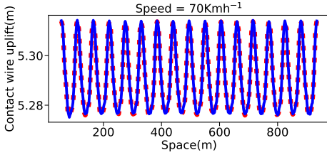
(a) Contact wire uplift prediction at 70 \text{ km h}^{-1}
