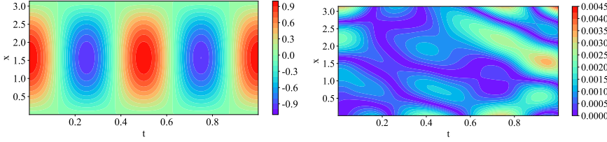
Figure 2.3: Nondimensional Euler-Bernoulli beam equation Color bar represents Left: Predicted solution ( u^* ); Right: Absolute error in prediction ( |u - u^*| )
