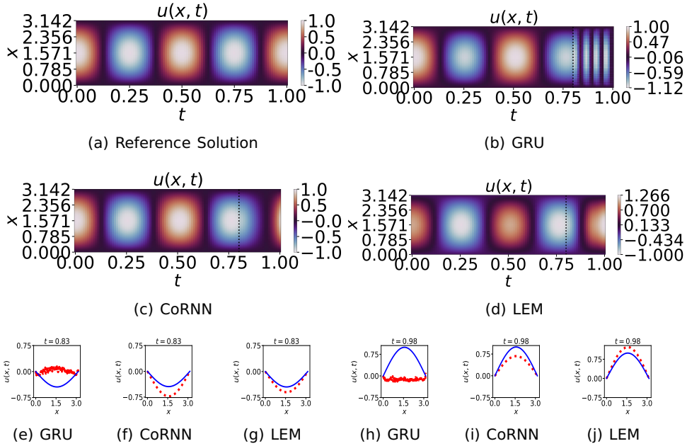
Figure 4.5: Top two rows: the complete reference solution and predictions for the Euler-Bernoulli beam equation. Bottom: the solution snapshots at t = \{0.83, 0.98\} obtained in the generalization region.
