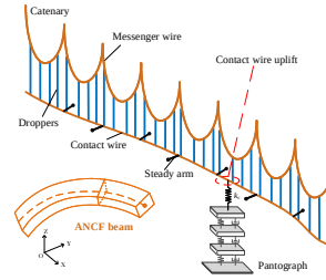
(b) Catenary-pantograph interaction simulation model. The Catenary is modeled by ANCF beam elements (contact and messenger wires) and cable elements (droppers). The pantograph is a lumped mass model with three degrees of freedom.
