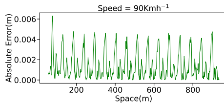
(f) Absolute error at 90 \text{ km h}^{-1}
