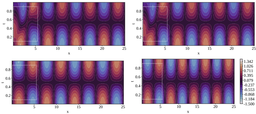
Figure 3.3: Euler-Bernoulli beam displacement on the Winkler foundation (Top Left.) Predicted solution using PINN (Top Right.) Predicted solution using SA-PINN (Bottom Left.) Predicted solution using causal PINN (Bottom Right.) Reference solution
