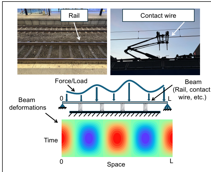
Figure 1.1: Examples of beams under varying transverse force. The direction of force on the rail is from above, whereas for the contact wire, it is from below. Different contour colors represent distinct space-time deformations of the beam and are not subject to scale.
