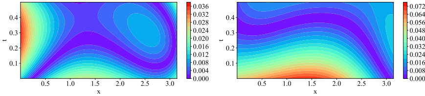
Figure 2.13: Timoshenko double-beam inverse problem: absolute error in the prediction of force when the additional data of rotation and deflections provided at five locations has left: no noise right: 20 percent Gaussian noise.
