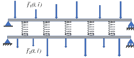
Figure 2.10: Double beam system connected by a Winkler foundation.
