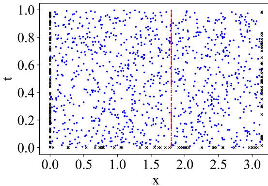
Figure 2.14: Data to learn material properties for the Timoshenko double beam: Blue dots Collocation points. Red dots Additional data points of displacement and rotation for the double beam at one location. Black dots Initial and boundary points.
