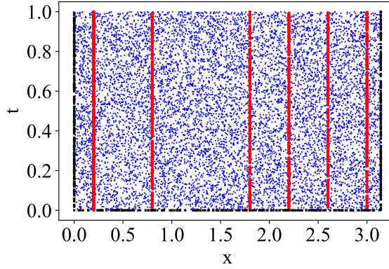
Figure 2.15: Data to learn force for the Timoshenko double beam: Blue dots Collocation points. Red dots Additional data points of displacement and rotation for the double beam at six different locations. Black dots Initial and boundary points.
