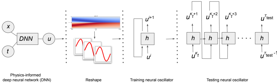
Figure 4.1: The proposed framework in which a physics-informed architecture (e.g., PINN or its variants) learns a solution in the convex hull X_1 . After reshaping, these solutions are represented sequentially and processed by one of the neural oscillators. The neural oscillator is finally tested in the convex testing hull X_2 , where the output of the last prediction step is the input for the next prediction step. Here, 1 \leq i \leq k_t , i \in \mathbb{Z} , and h = [y, z] . The dotted lines separate different stages of training and testing the framework.
