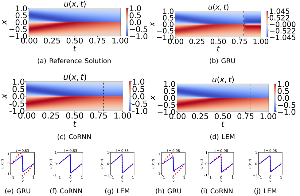
Figure 4.2: Top two rows: the complete reference solution and predictions for viscous Burgers equation. The black vertical line delineates the region before which the PINN has been trained. The region after the black vertical line represents the generalization domain. The meaning of the vertical line remains the same in the following figures. Bottom: the solution snapshots at t = \{0.83, 0.98\} obtained in the generalization region, where blue represents the reference solution, and red refers to the recurrent method. The colors are used consistently for the following figures.
