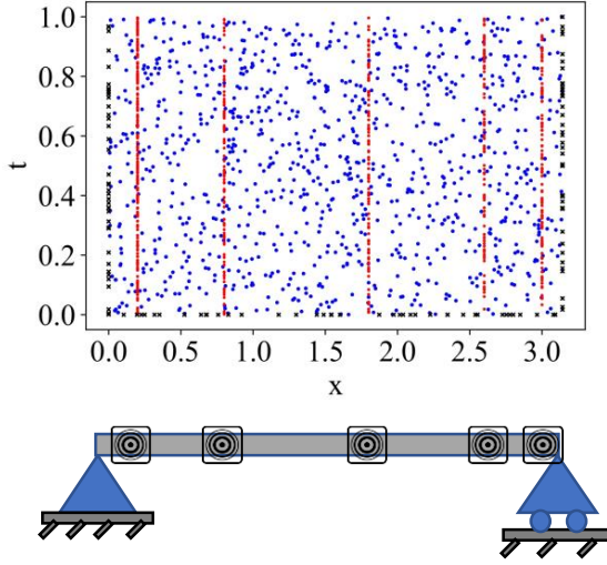
Figure 2.7: Data to learn the parameters for the Timoshenko single-beam: Blue dots Collocation points. Red dots Additional data points of rotations ( \theta ) and displacement ( u ). Black dots Initial and boundary points.
