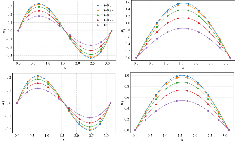
Figure 2.11: Timoshenko double beam. Scattered points represent the exact solution, and the continuous line refers to the predicted solution. Top: First beam Left Displacement ( w_1 ); Right Rotation ( \theta_1 ). Bottom: Second beam Left Displacement ( w_2 ); Right Rotation ( \theta_2 )
