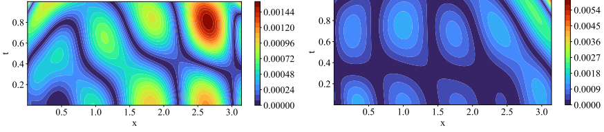
Figure 2.6: Timoshenko single beam absolute error in predictions Left: |\theta - \theta^*| ; Right: Absolute error |w - w^*| .
