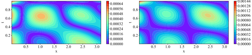
Figure 2.8: Euler-Bernoulli double-beam: color bar represents absolute error in predictions Left: |w_1 - w_1^*| ; Right: |w_2 - w_2^*| .
