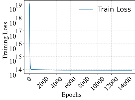
Figure 2.2: L-BFGS training loss vs. the number of epochs for the dimensional Euler-Bernoulli beam equation.
