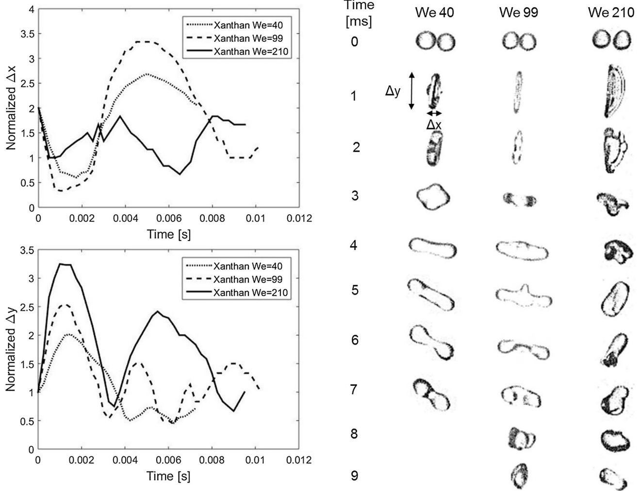
Fig. 11 Evolution in time of the two axial sizes of the collisional complex for xanthan with B=0 and for the cases We = 40 , We = 99 , and We = 210
