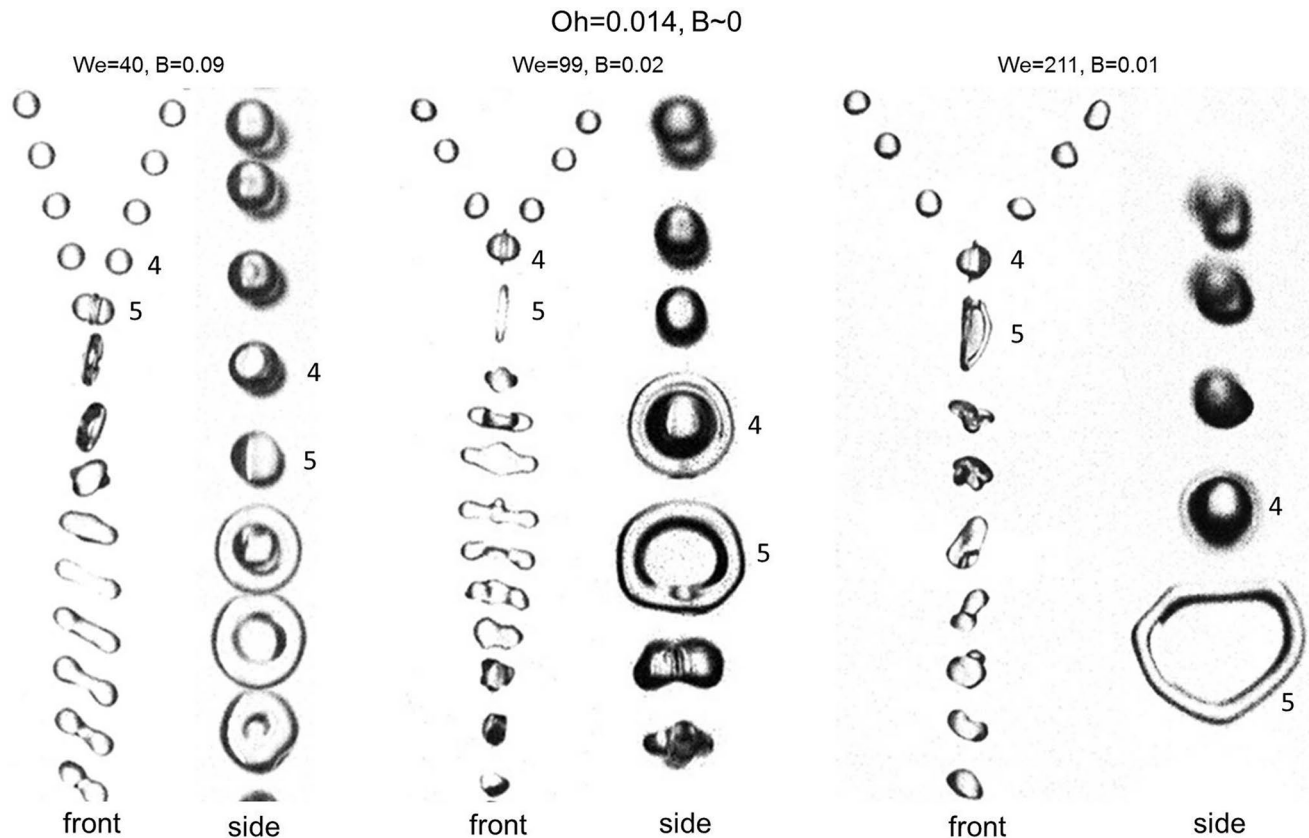
Fig. 6 Three droplet collisions for xanthan at We = 40, 99 , and 211 and an impact parameter B close to zero. Note that the droplets seen in a collision example are the same, in both the side camera and front camera frame
