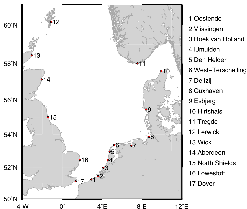
Figure 1. Location of the 17 tide gauge stations around the North Sea.
