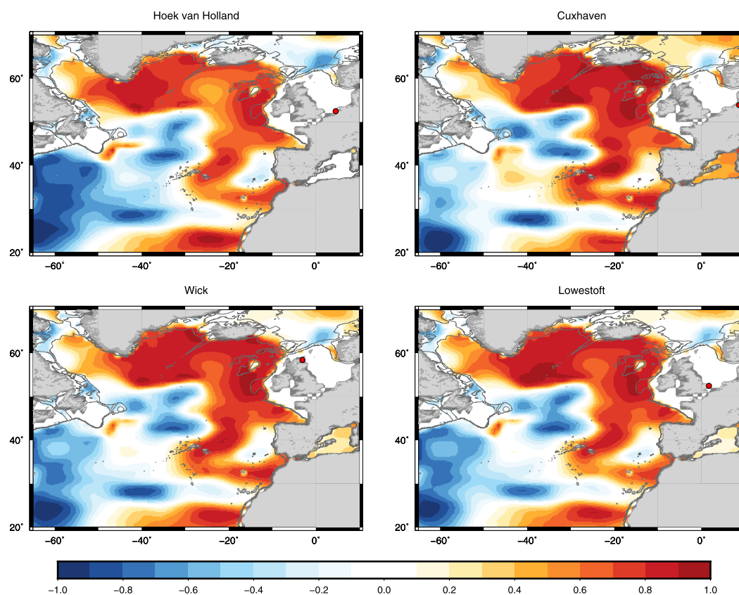
Figure 9. Correlation between time-varying trend in steric sea level and the time-varying sea level trend from model C for four North Sea stations. The 250 and 1000 m isobaths are shown in grey. No correlation is shown for grid points at a depth smaller than 250 m. The averaged time-varying trend for each station and each grid point has been removed using equation (43).
