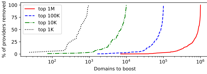
Fig. 5. The percentage of fingerprinting script providers that would not be detected if a given number of domains were pushed above all fingerprinting domains for different subsets of Alexa’s ranking.
