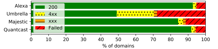
Fig. 4. The responsiveness and reported HTTP status code across the lists.
