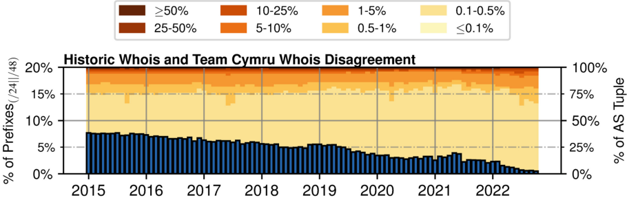
Fig. 2. Percentage of prefixes in the dataset on which the historic whois service we implemented and the data from Team Cymru’s bulk whois service disagree. The shaded background indicates the distribution of disagreement over AS tuple, i.e., the tuple of the ASes to which Team Cymru attributes a prefix and the ASes BTTF attributes a prefix to. Note that, as common with centralization, only a minor fraction of AS tuples is responsible for the bulk of disagreement.
