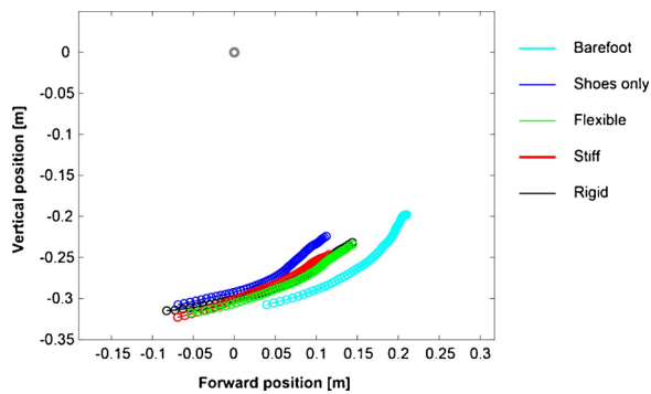
Fig. 1. Mean RoS (n = 15), normalized for shank length, during single support for different walking conditions. Grey dot indicates the lateral epicondyle, i.e. origin of the shank's local reference frame.
