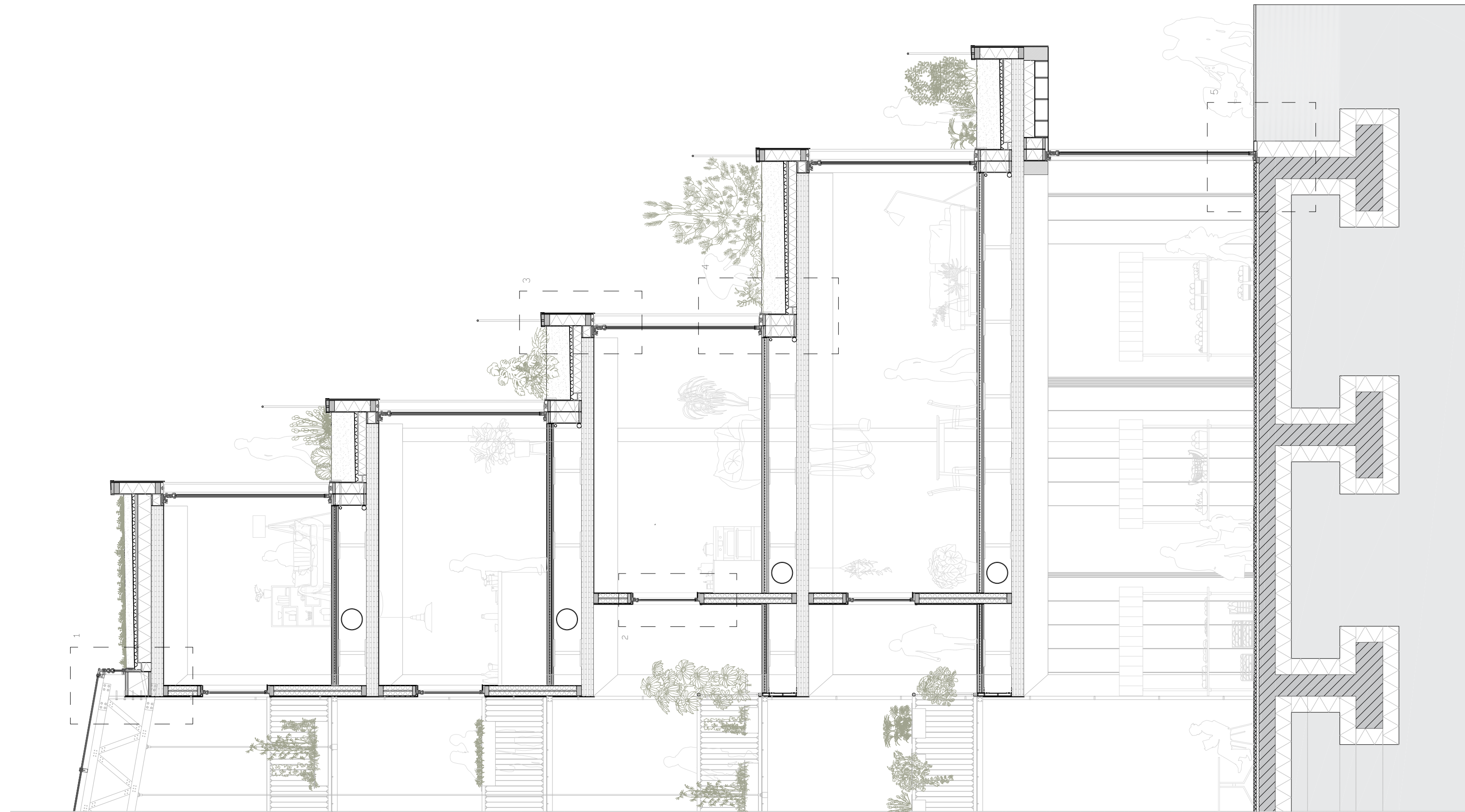
Overview detailing South facade
