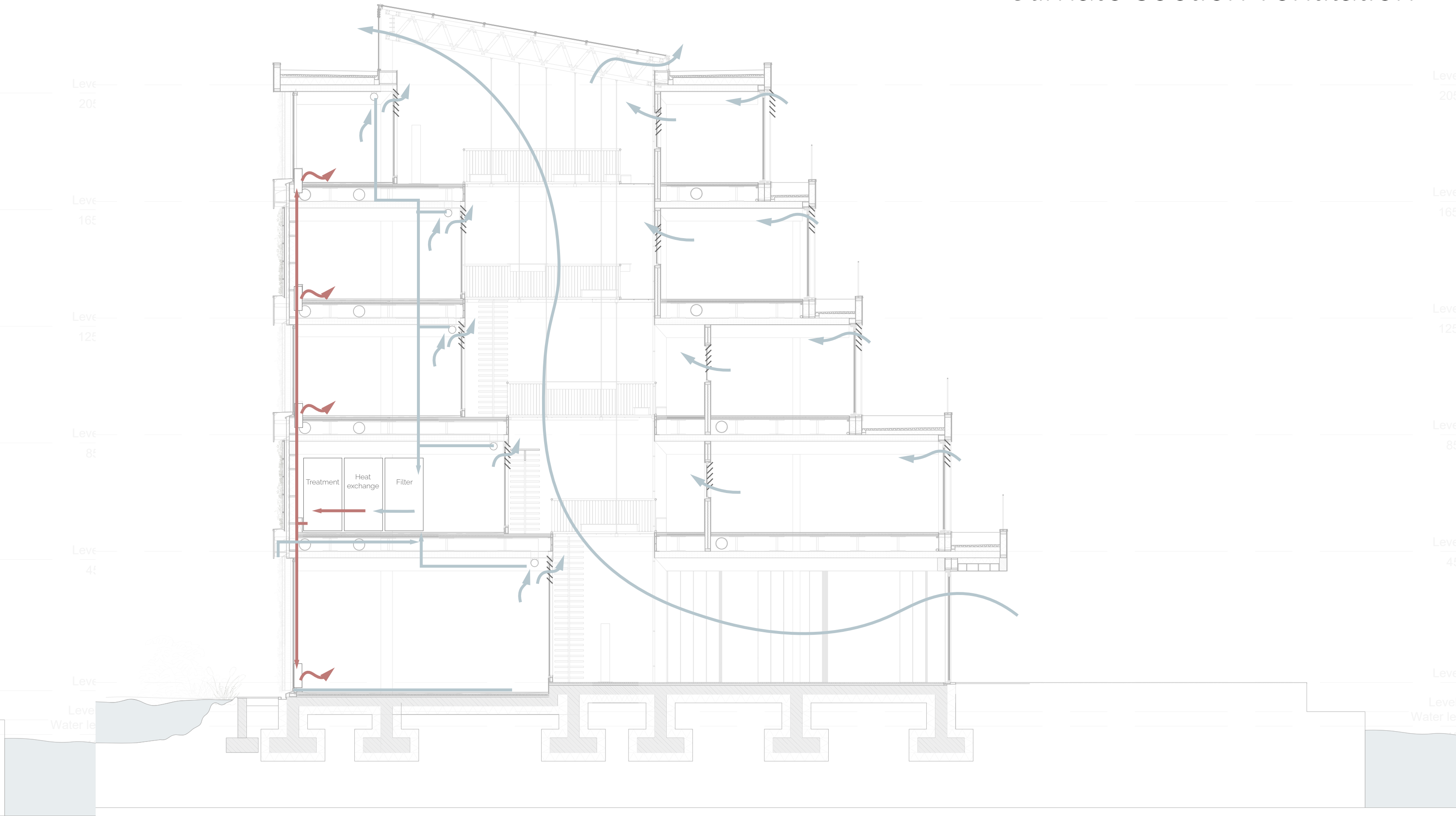
Climate section ventilation
