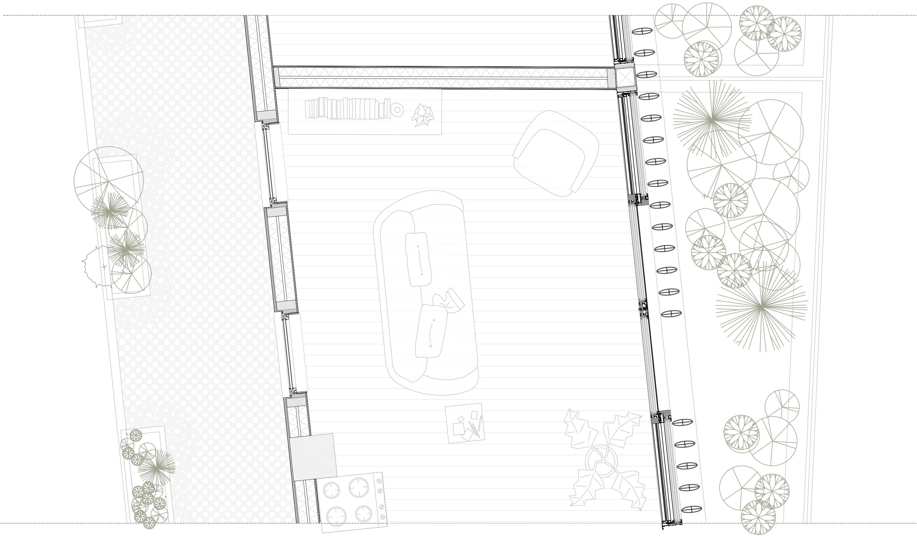
1-20 South facade horizontal fragment
