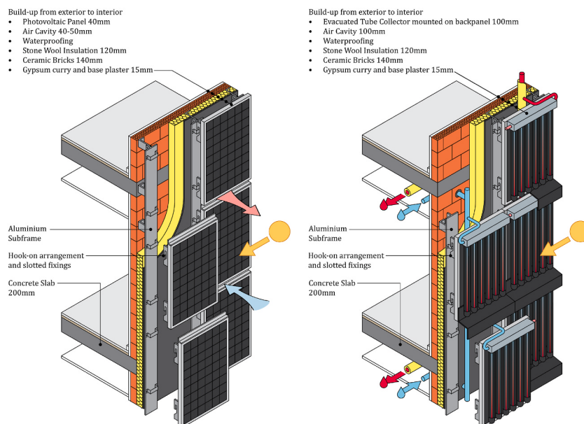
Fig. 8. Demonstration of a detailed design of the PV façade (left side) and the ETC façade (right side).
