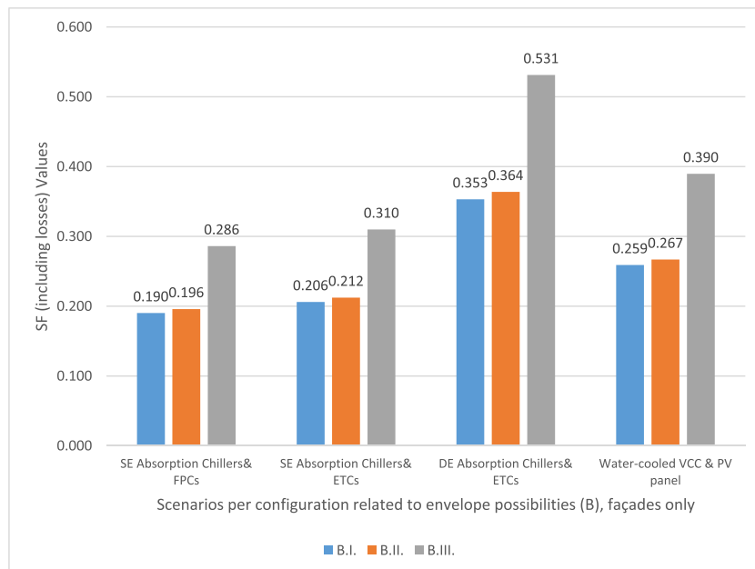
Fig. 4. SF values (including losses) for scenarios related to envelope possibilities (B), façades only.
