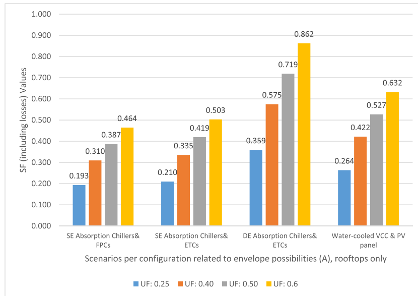
Fig. 3. SF values (including losses) for scenarios related to envelope possibilities (A), rooftops only.
