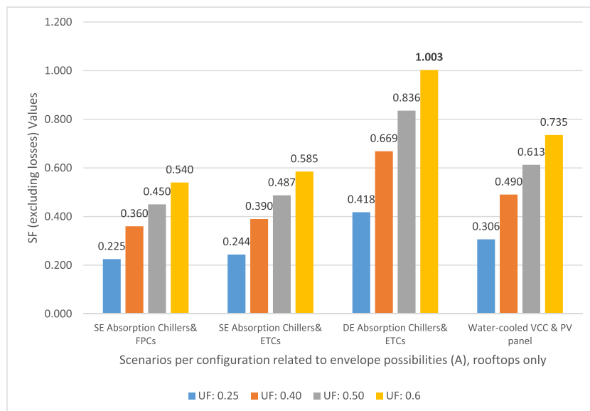
Fig. B.2. SF values (excluding losses) for scenarios related to envelope possibilities (A), rooftops only.
