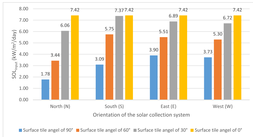
Fig. B.1. Daily average solar irradiance SOL_{input} at different orientations of the solar collection system considering the month of summer design week
