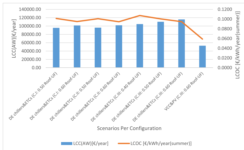
Fig. 6. Cost-effectiveness based on LCC_{AW} and LCOC for scenarios involving Double-Effect (DE) absorption chillers with Evacuated Tube Collectors (ETCs) (thermally driven) and water-cooled VCC and PV panels (electrically-driven), considering those with Solar Fraction (SF) values of 1 or higher.
