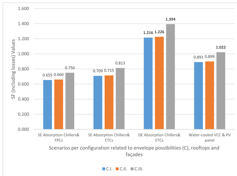
Fig. 5. SF values (including losses) for scenarios related to envelop possibilities (C), rooftops and façades.
