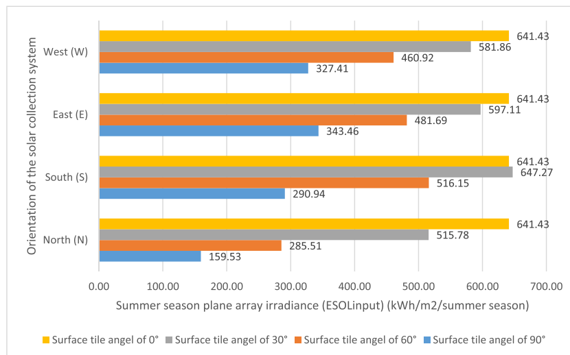
Fig. B.3. Plane array irradiance available on a particular location/orientation considering whole summer as the time frame ESOL input
