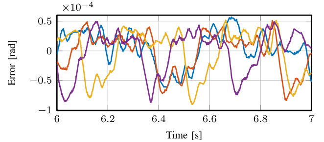
Fig. 8. Measurement of the error as a function of time for different velocities 0.08 rad/s (—), 0.1 rad/s (—), 0.12 rad/s (—) and 0.14 rad/s (—), which are all periodic but with different period.
