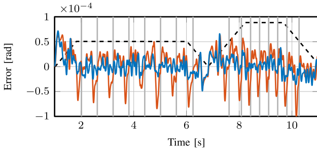
Fig. 19. Experiment with a varying velocity in (---) (scaled), for the state-of-the-art feedback controller (orange) and with the learned GP-based compensation function in (blue).
