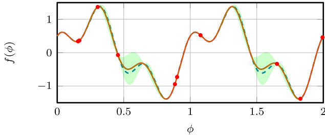
Fig. 11. Example 1: Gaussian process regression is performed with 10 random samples (f(\phi_i), \phi_i) denoted by (\bullet) taken from the true periodic function \bar{d}(\phi) ( - - ). The resulting GP f(\phi) has posterior mean ( - ) and posterior variance ( \text{shaded green} ), which is a good estimate of \bar{d}(\phi) also in-between training points by selecting appropriate smooth and periodic prior knowledge.
