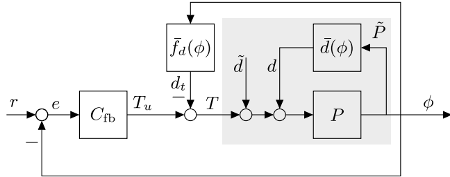
Fig. 4. Torque ripple compensation strategy where the aim is to learn the compensation function \tilde{f}_d(\phi) from data. The CPA is modeled as \tilde{P} with non-linearity \tilde{d}(\phi) that is spatially periodic such that d(k) represents a torque ripple or commutation-induced disturbance, and additional non-repeating disturbances \tilde{d} .
