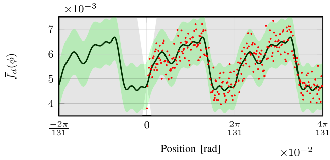
Fig. 18. Learned GP-based compensation function \tilde{f}_d with 99.7% confidence bound (green), which is trained with data that is obtained with the RC experiment at 0.1 rad/s. The sector bound condition (17) with \rho = 0.5 is shown in (grey).
