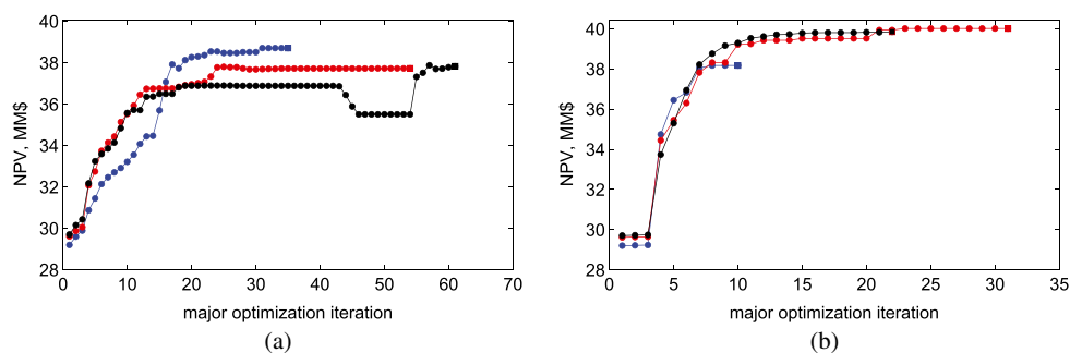
Fig. 7 NPV as a function of major optimization iterations for a constrained optimization and b optimization with constrained simulations; all simulations performed for small (black), medium (red), and large (blue) time step refinements after control update
